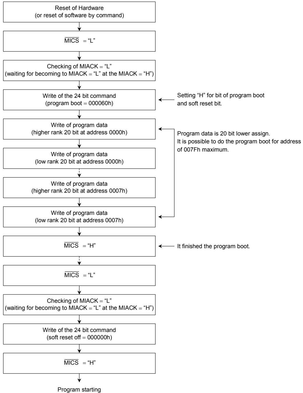
Figure 2 Procedure of Program Boot and Program Start
