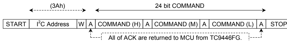
Figure 10 Format Only a Command at the Time of Transmission.
