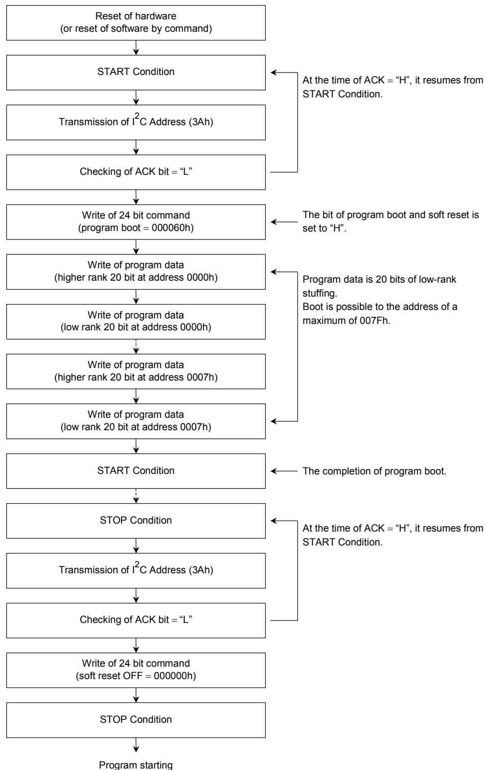
Figure 11 Procedure of Program Boot and Program Start
