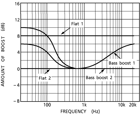
Note : Bass boost 2 matches with flat 2 when 1kHz or more Fig.6 Bass boost characteristics
