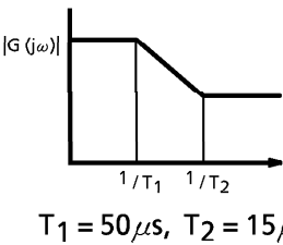
Fig.5 Filter characteristics
