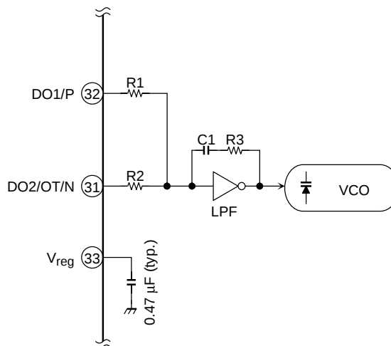
When LPF is used in common (Set DO2 as high impedance and switch the filter constant)
