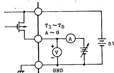
TEST CIRCUIT (2)
