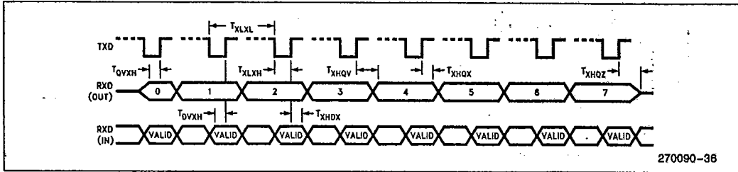
SERIAL PORT WAVEFORM—SHIFT REGISTER MODE
