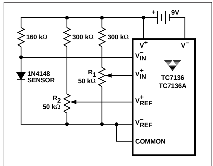
Figure 13. Temperature Sensor
