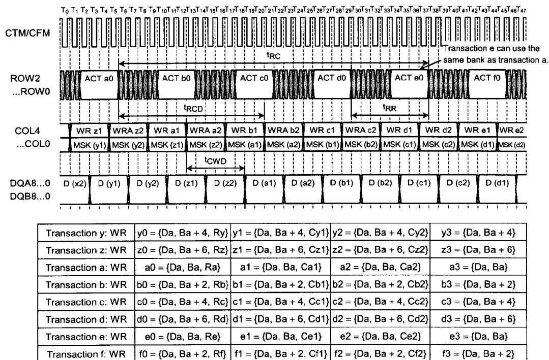
Figure 21. Interleaved Write Transaction with Two Dualocts Data Length
