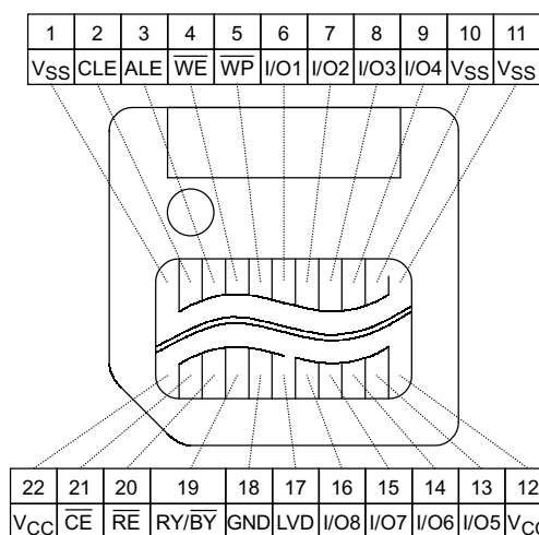
Figure 1. Pinout
