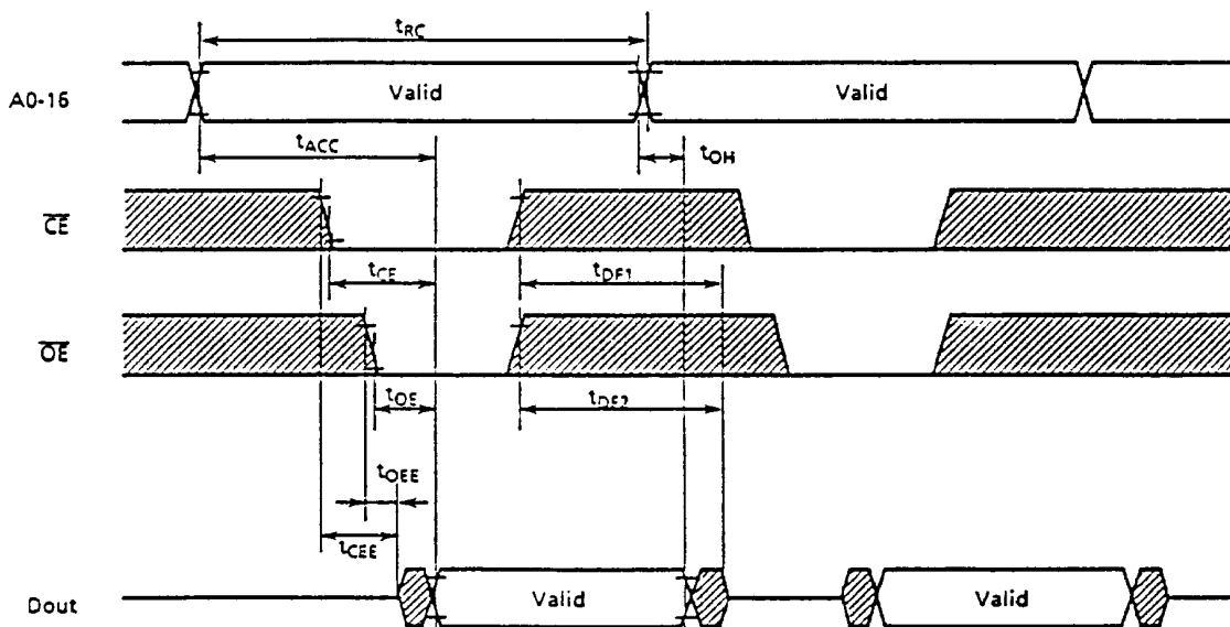
Timing Waveform of Read Cycle
