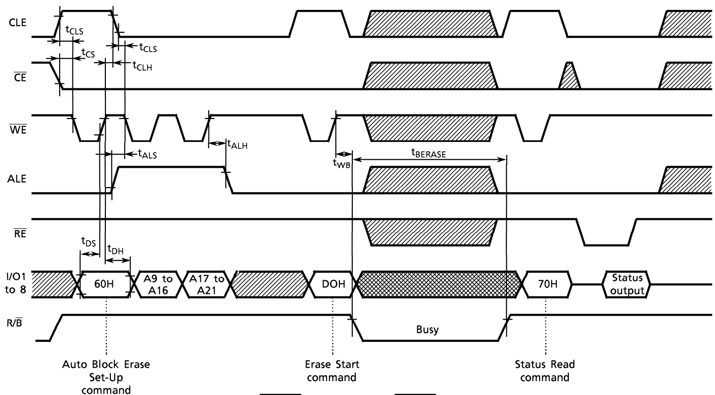
Auto Block Erase Timing Diagram
