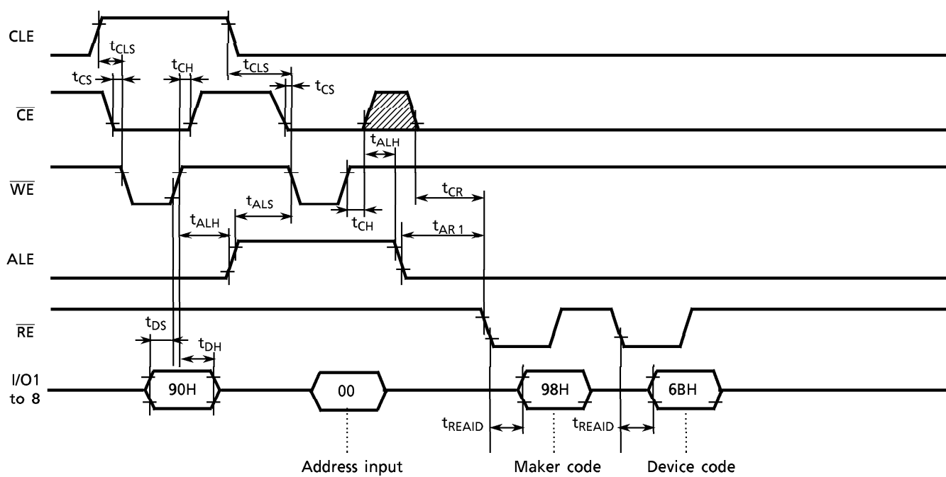
ID Read Operation Timing Diagram
