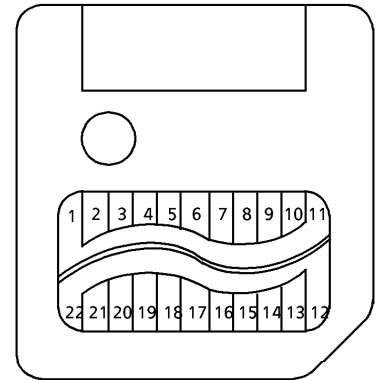
Figure 1. Pinout
