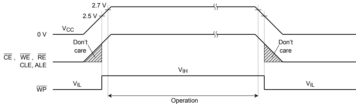
Figure 15. Power-on/off Sequence
