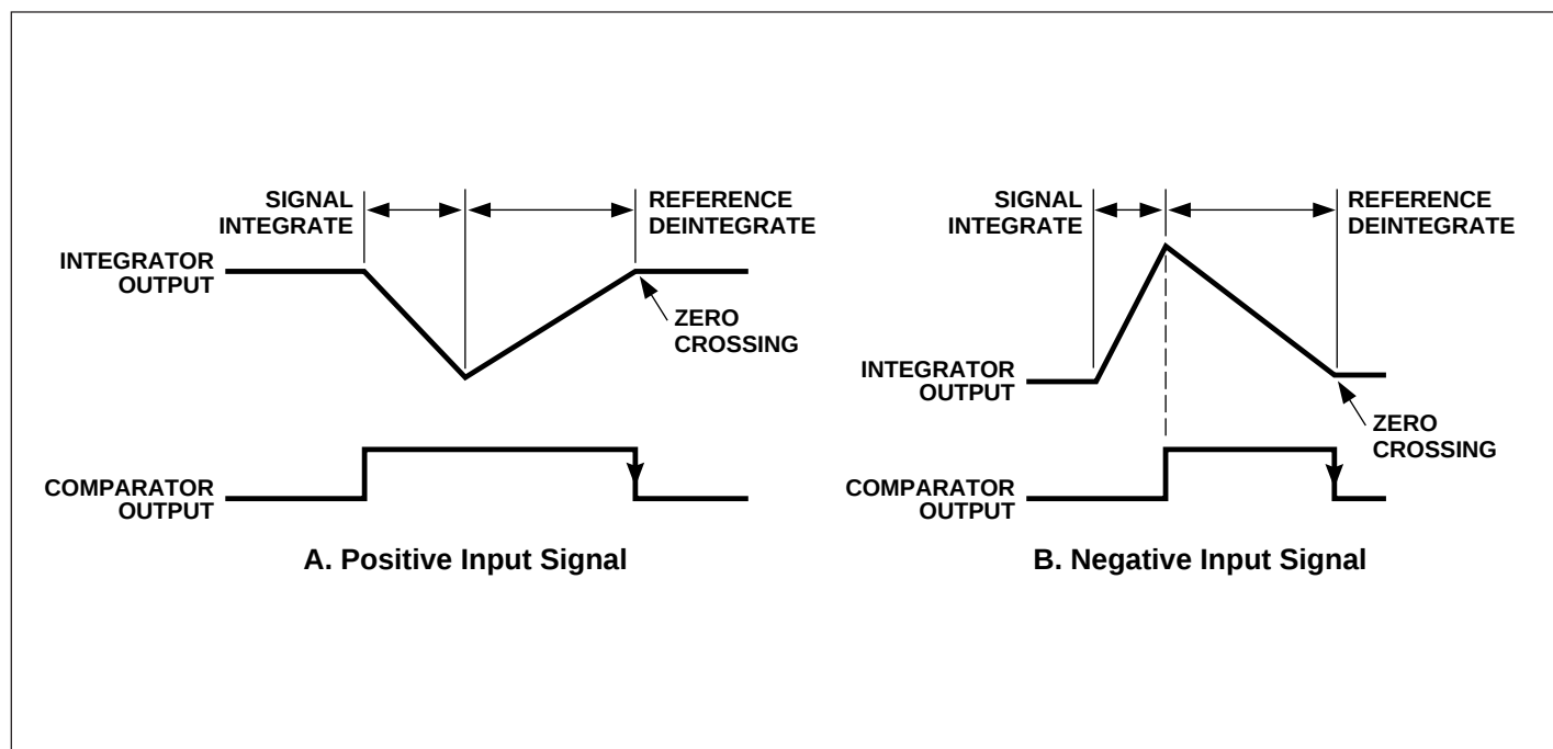
Figure 5. Comparator Output
