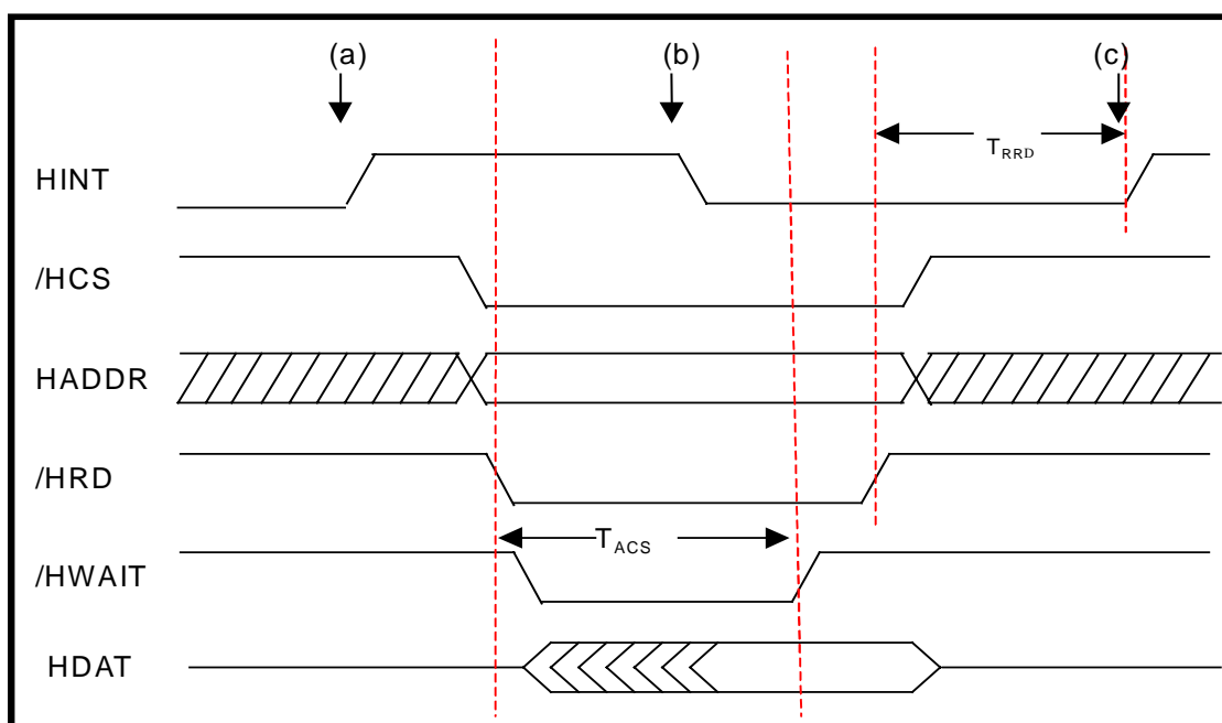
Fig. 7 Interrupt Operation
