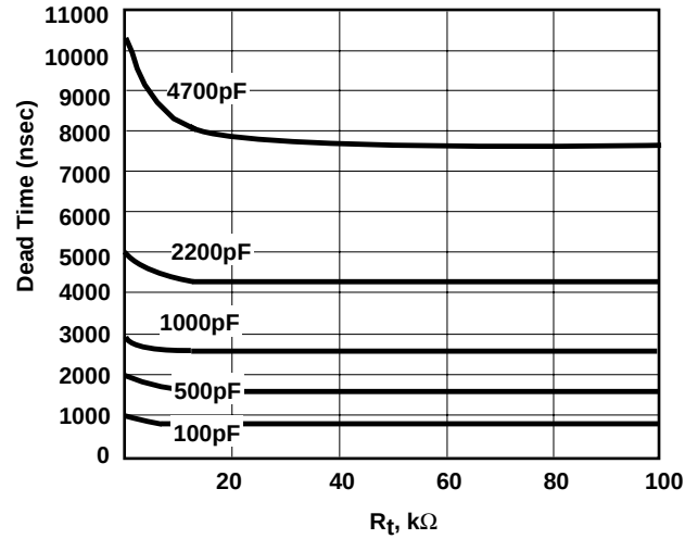
18C46 Dead Time vs. R_t
