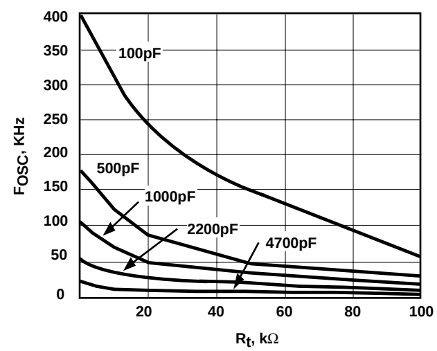
18C46 OSC Frequency vs. R_t
