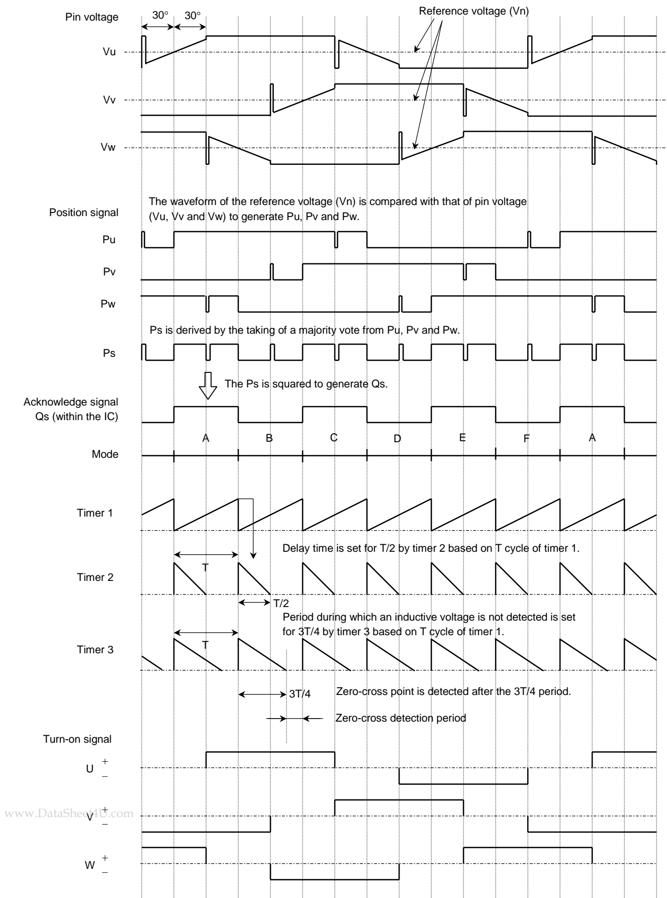
Figure 1 Sensorless drive timing chart (lead angle: 0°)
