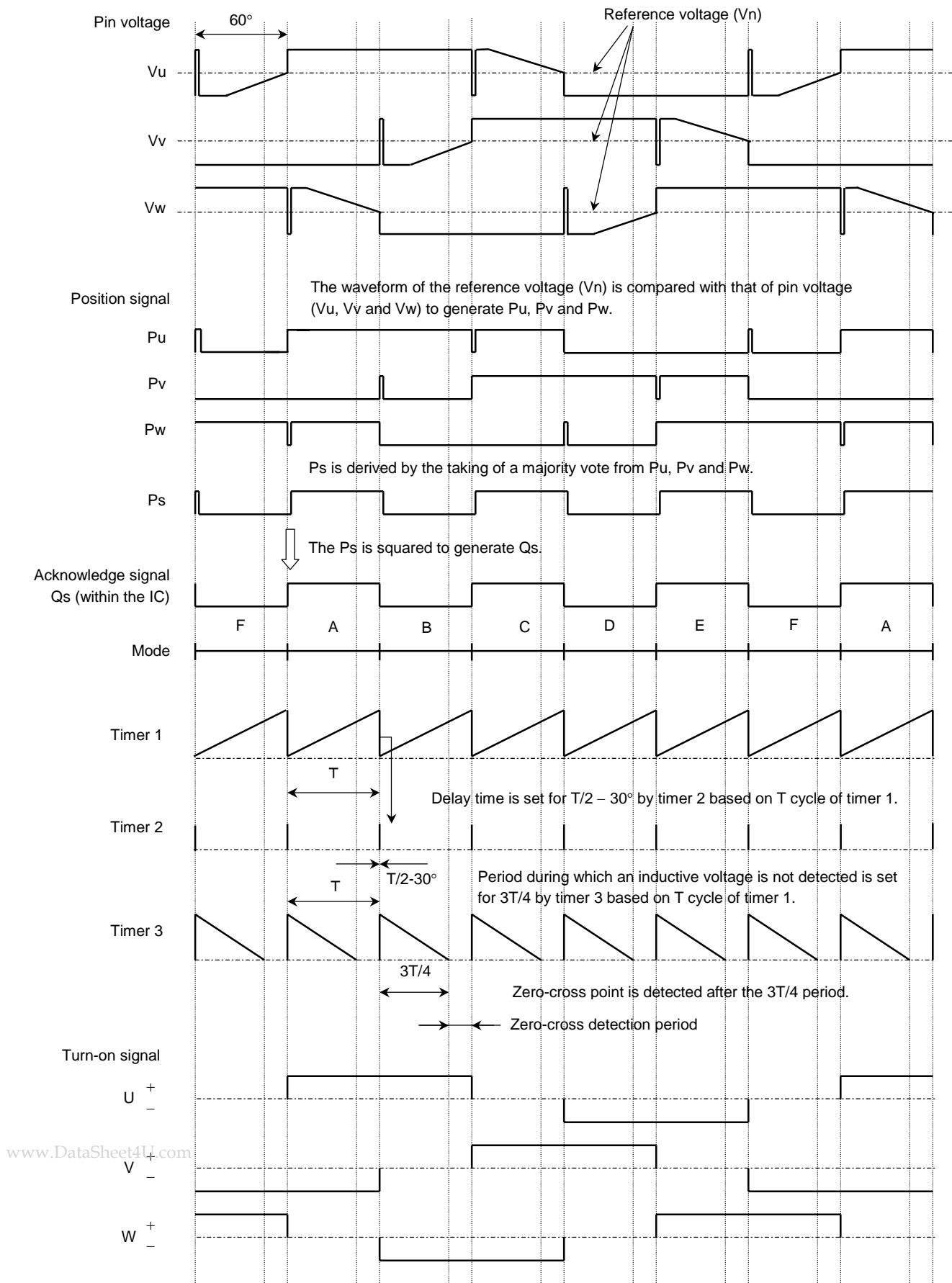
Figure 4 Sensorless drive timing chart (lead angle: 30°)
