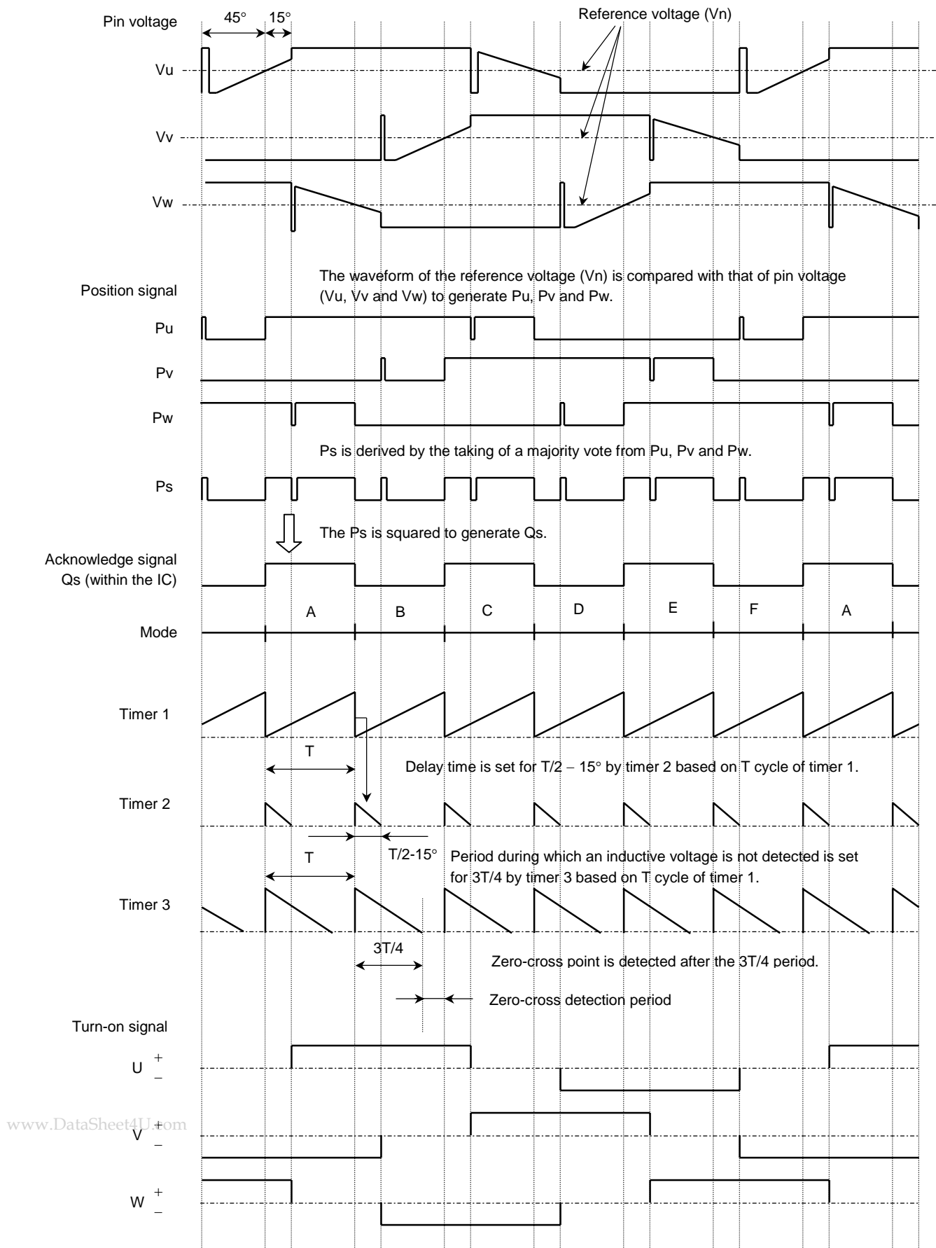
Figure 3 Sensorless drive timing chart (lead angle: 15°)
