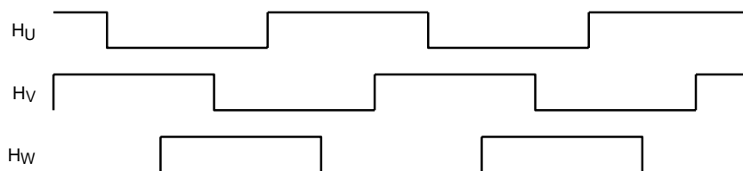
Output waveform
