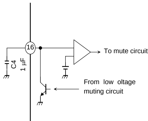
Figure 2 Pin 16 Muting Circuit
