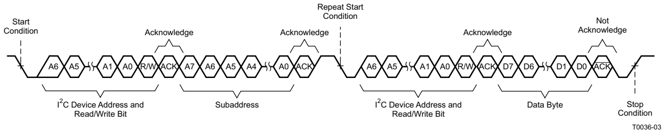
Figure 52. Read Transfer
