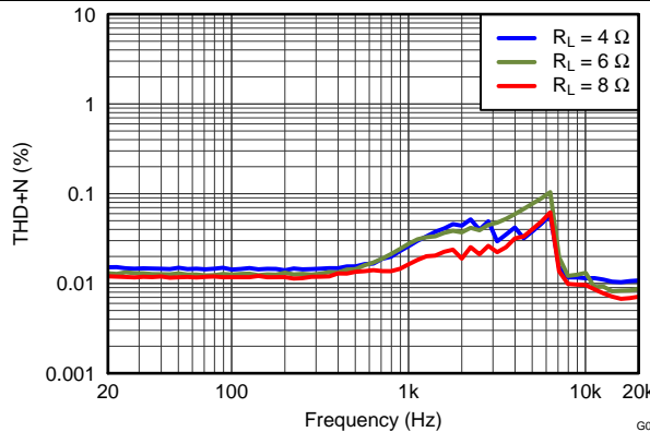
PVDD = 24 V, P_{\text{OSPK}} = 1 \text{ W} Figure 3. THD+N vs Frequency
