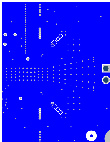
Figure 75. Layout Example (Mono) - Bottom Layer
