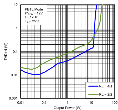
Figure 34. Total Harmonic Distortion + Noise vs Output Power (PBT Mode)
