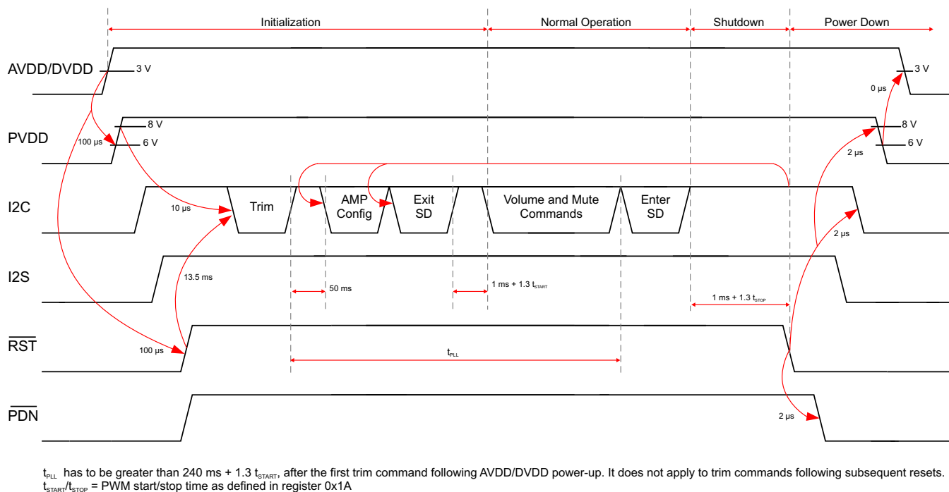
Figure 68. Recommended Start-Up and Shutdown Sequence
