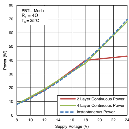
Figure 33. Output Power vs Supply Voltage (PBT Mode)
