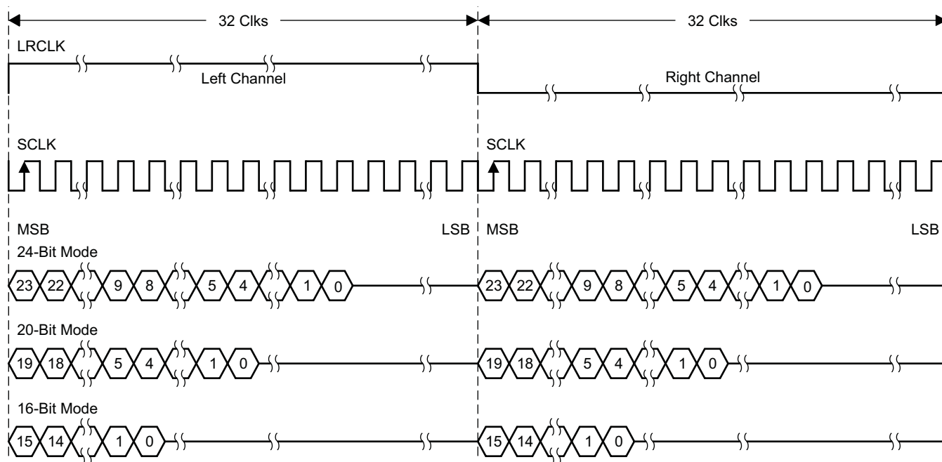
Figure 58. Left-Justified 64- f_s Format
