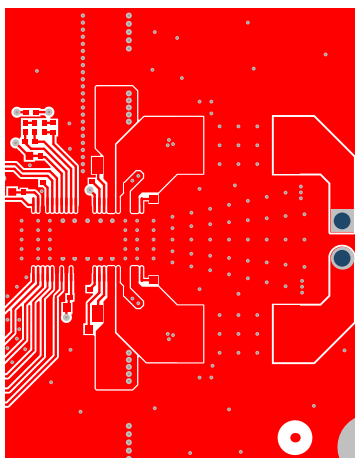
Figure 74. Layout Example (Mono) - Top Layer
