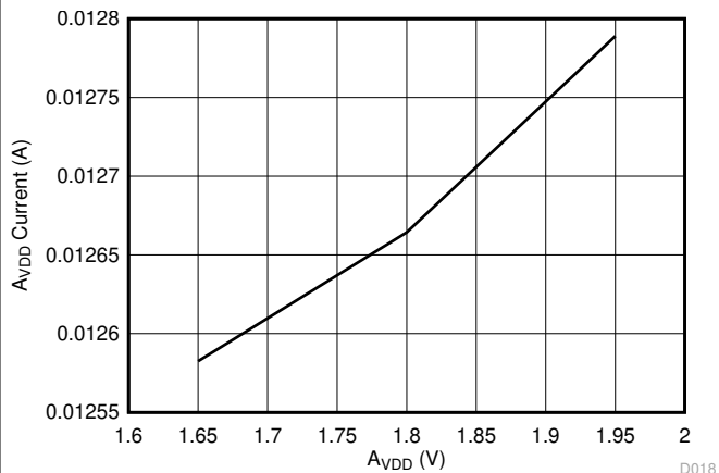
Figure 6-18. A_{VDD} Idle Current vs A_{VDD}
