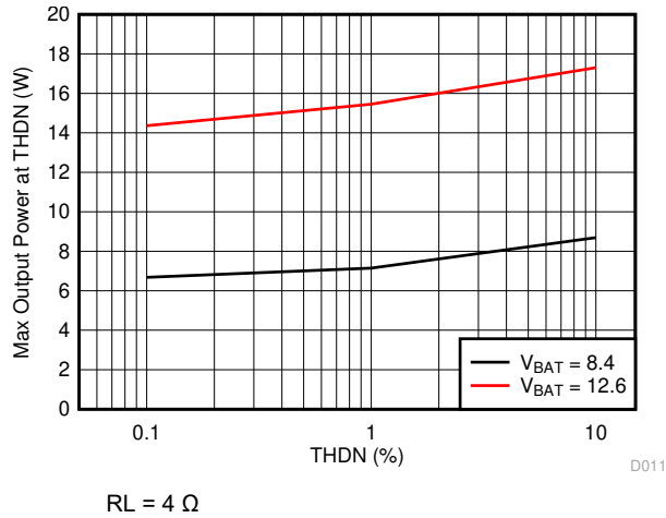
Figure 6-11. Max Output Power vs THD+N
