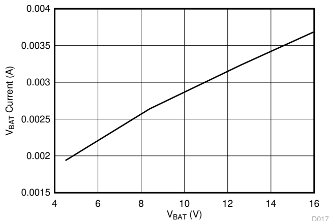
Figure 6-17. V_{BAT} Idle Current vs V_{BAT}
