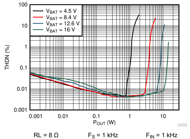
Figure 6-2. THD+N vs Output Power
