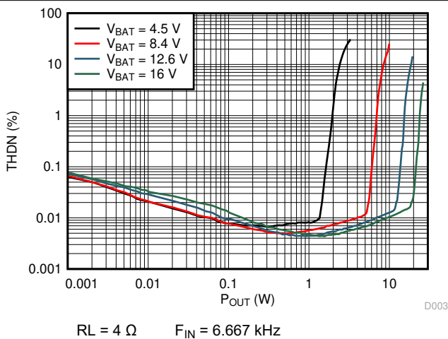
Figure 6-3. THD+N vs Output Power
