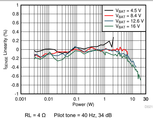
Figure 6-21. I_{SENSE} Gain Linearity vs Output Power
