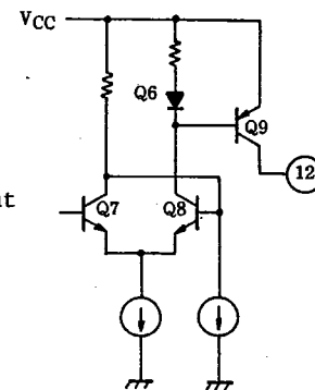
Fig.3 TERMINAL TO STOP VCO
