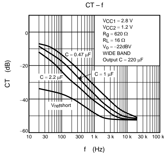
Figure 6 Low-Pass Compensation Condenser and Crosstalk
