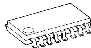
SSOP16-P-225-1.00A
