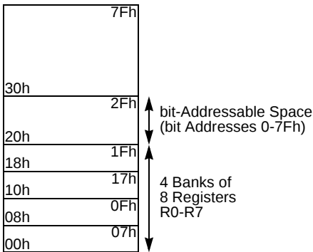
Figure 10. Lower 128 Bytes Internal RAM Organization
