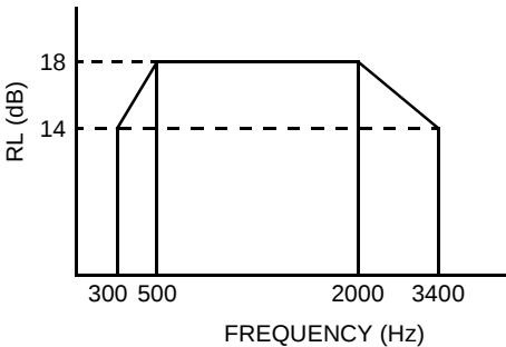
Figure 8. Return Loss
