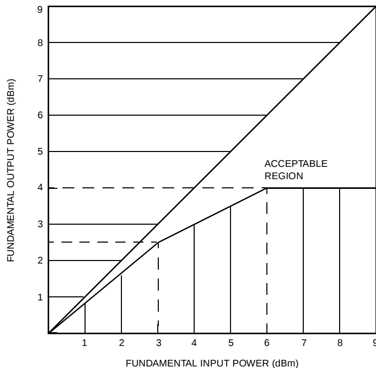
Figure 4. Overload Compression
