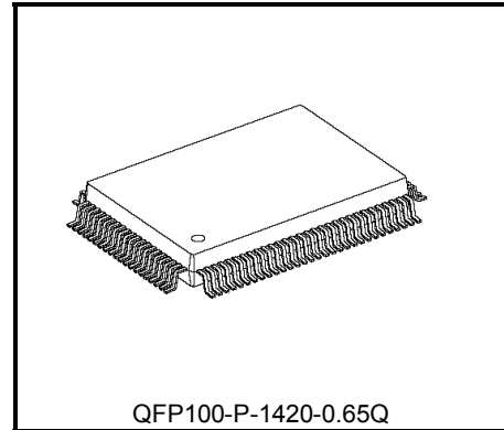
QFP100-P-1420-0.65Q Weight: 1.6 g (typ.)
