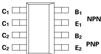
PARTMARKING DETAIL – T6790
