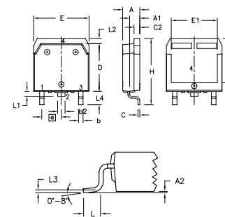
TO-268 Outline
