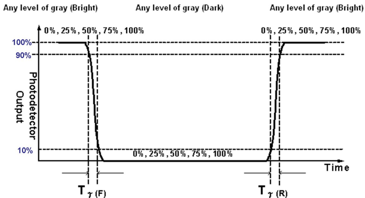
FIG. 2 Luminance
