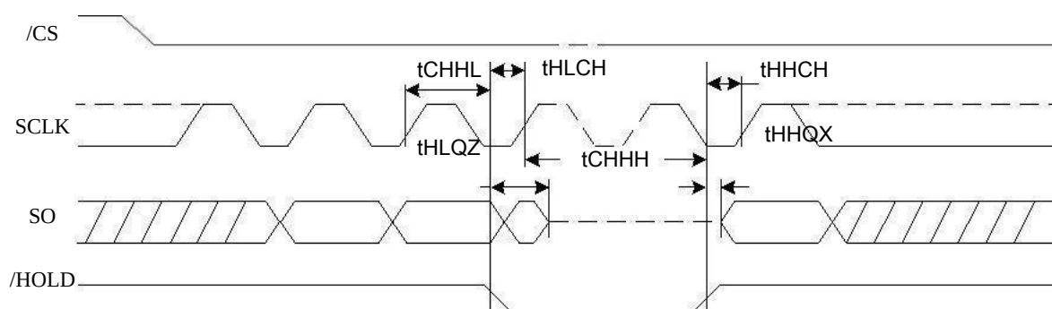
Figure 38. Hold Timing
