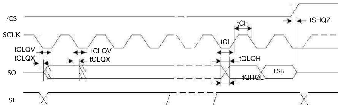
Figure 37. Output Timing
