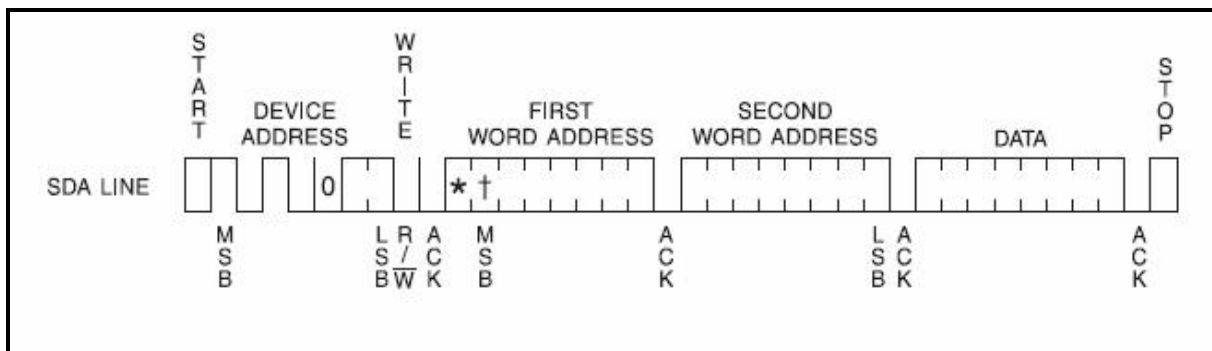
Figure 6. Page Write
