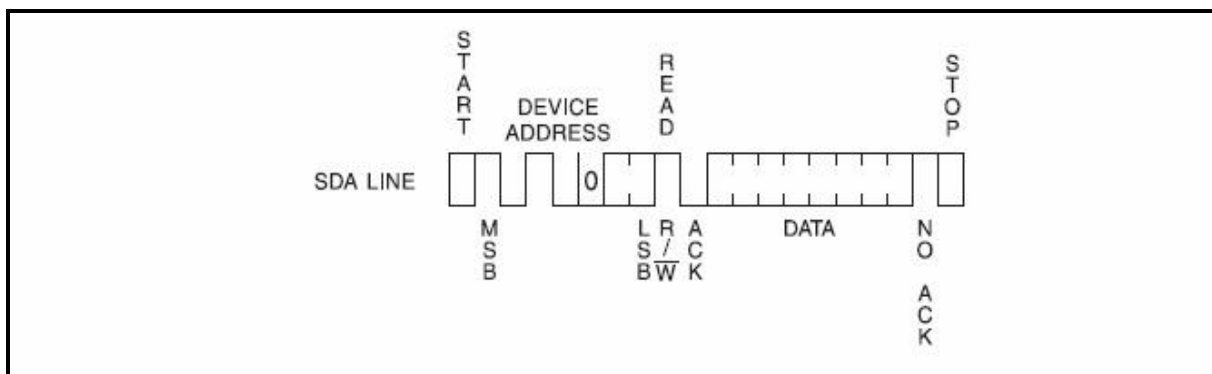
Figure 8. Random Read
