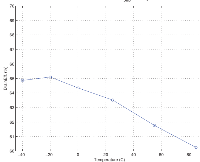
Drain Efficiency vs. Temperature 3300 MHz, 28V, 50 mA; CW P_{3dB} Compression
