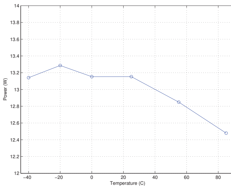
Power vs. Temperature 3300 MHz, 28V, 50 mA; CW P_{3dB} Compression
