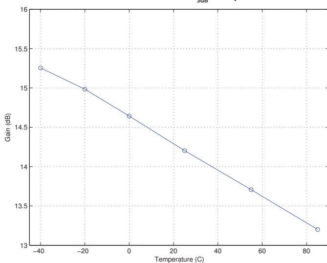
Gain vs. Temperature 3300 MHz, 28V, 50 mA; CW P_{3dB} Compression
