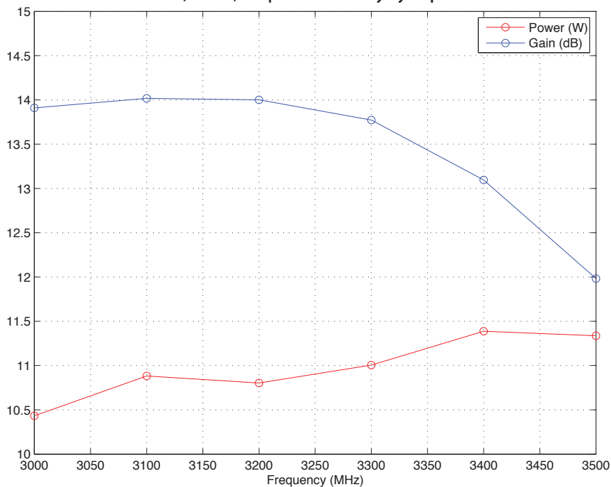
T1G6000528-Q3 P3dB Compression in Narrowband Fixture 28V, 50mA; 200μsec – 20% duty-cycle pulse
