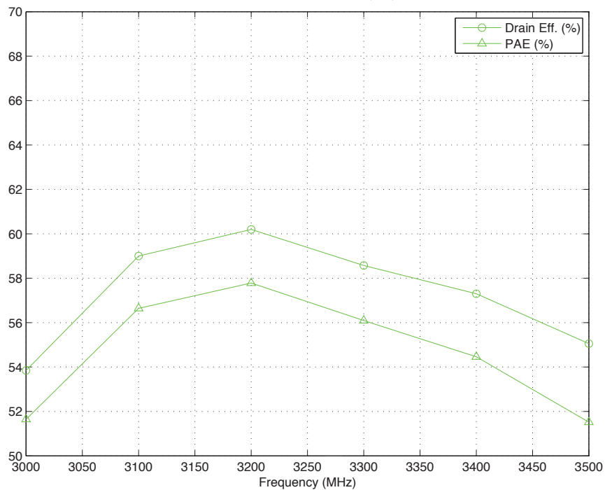
T1G6000528-Q3 P3dB Compression in Narrowband Fixture 28V, 50mA; 200μsec – 20% duty-cycle pulse
