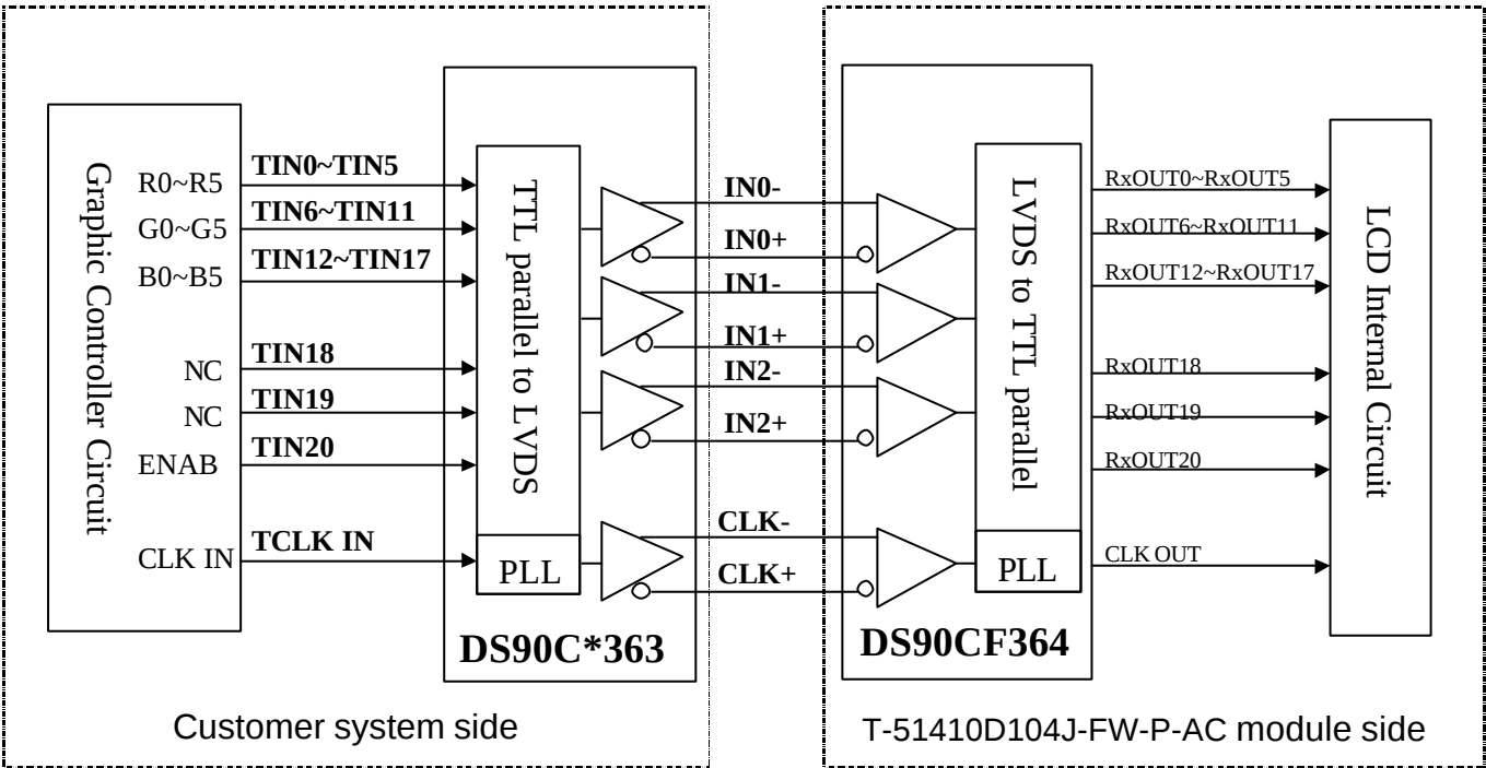
LVDS Interface Block Diagram
