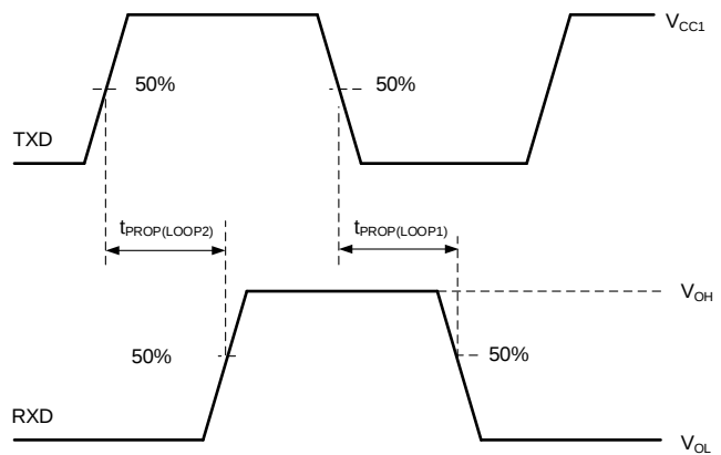
Figure 8. t_{\text{LOOP}} Test Circuit and Timing
