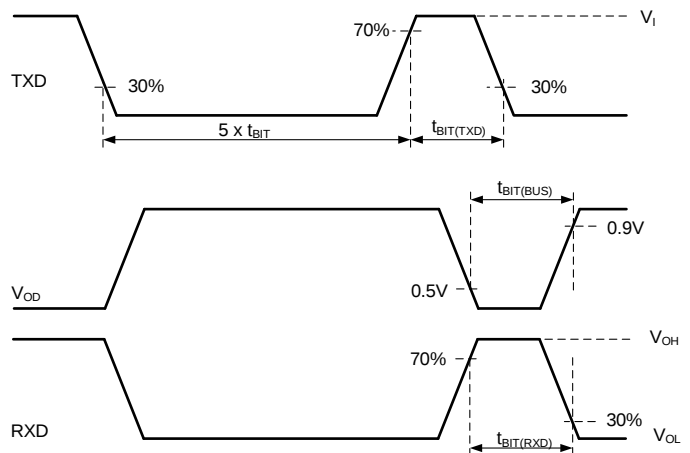
Figure 9. CAN FD Test Circuit and Timing
