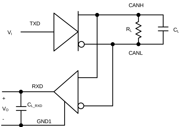
Figure 8. t_{\text{LOOP}} Test Circuit and Timing
