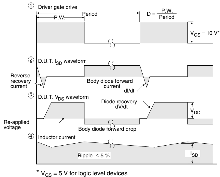
Fig. 16 - For N-Channel
