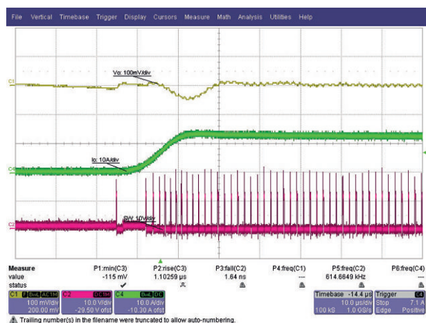
Fig. 28 - Load Step, 0.1 A to 12 A, 1 A/ \mu s, t = 10\text{ }\mu s/div Skip Mode Enabled
