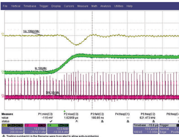
Fig. 29 - Load Step, 0.1 A to 12 A, 1 A/ \mu s, t = 10\text{ }\mu s/div Forced Continuous Conduction Mode
