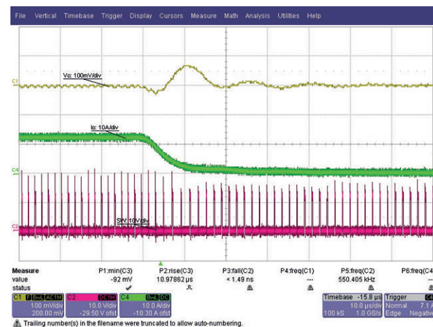
Fig. 32 - Load Release, 12 A to 0.1 A, 1 A/ \mu s, t = 10\text{ }\mu s/div Forced Continuous Conduction Mode
