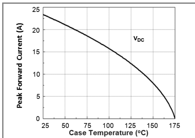
Fig.6 Current Derating
