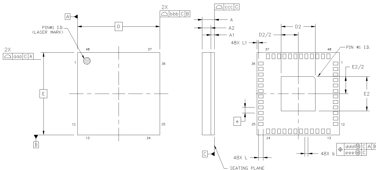
Figure 7.4. 48-Pin LGA
