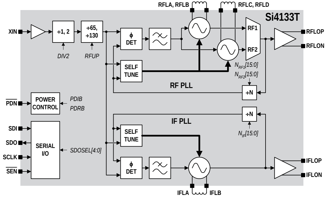
Figure 15. Si4133T Frequency Synthesizer Block Diagram
