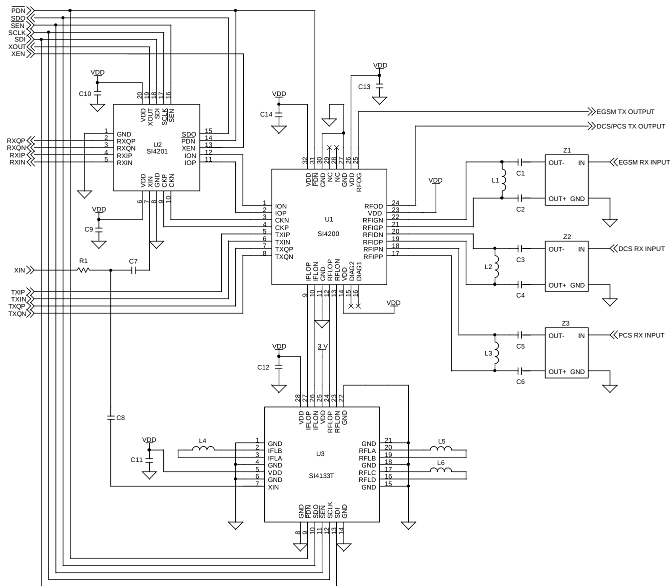
Figure 11. Typical Triple-Band Application Circuit
