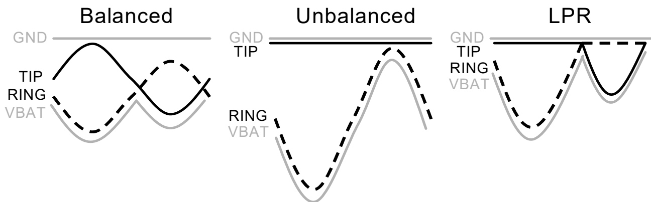
Figure 21. Ringing Modes
