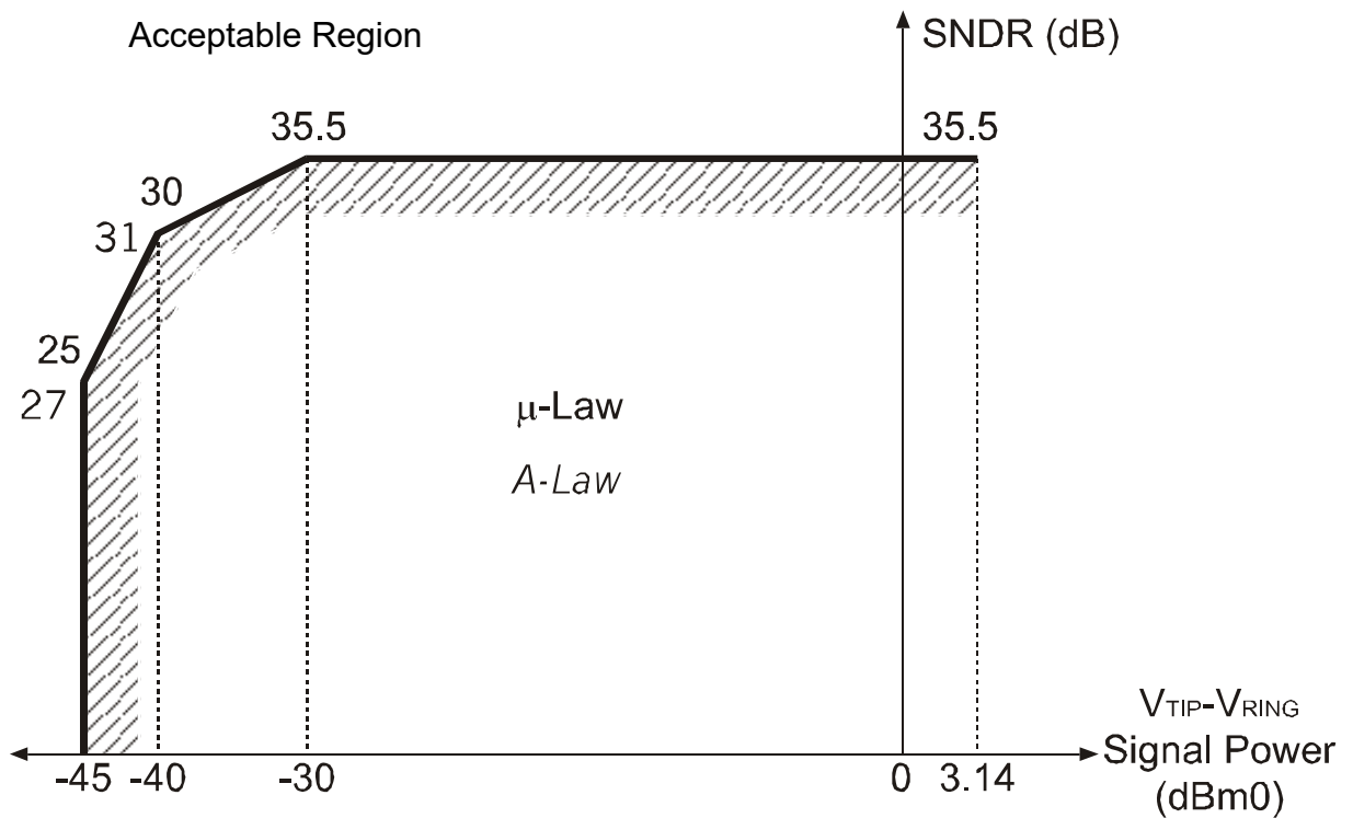
Figure 14. Transmit and Receive Path SNDR
