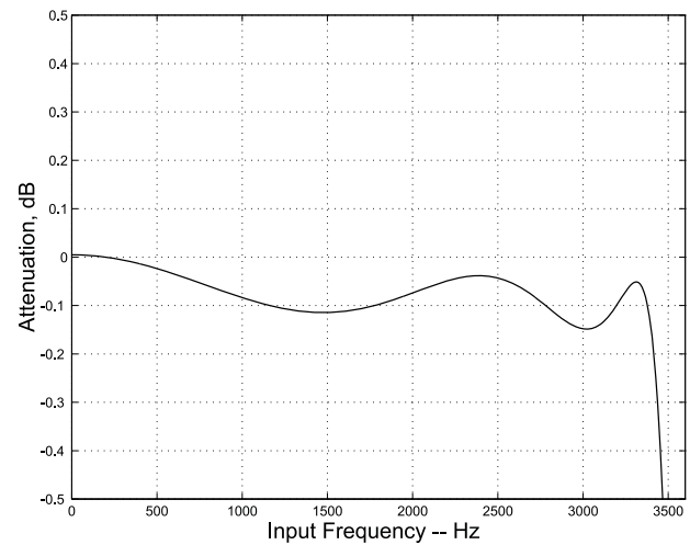
Figure 7. IIR Receive Filter Passband Ripple
