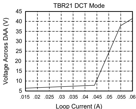
Figure 24. TBR21 Mode I/V Characteristics
