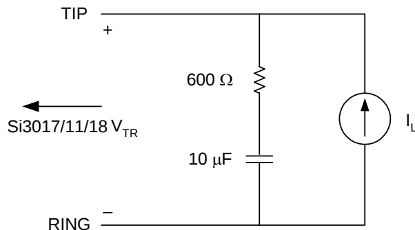
Figure 2. Test Circuit for Loop Characteristics
