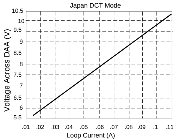
Figure 25. Japan Mode I/V Characteristics
