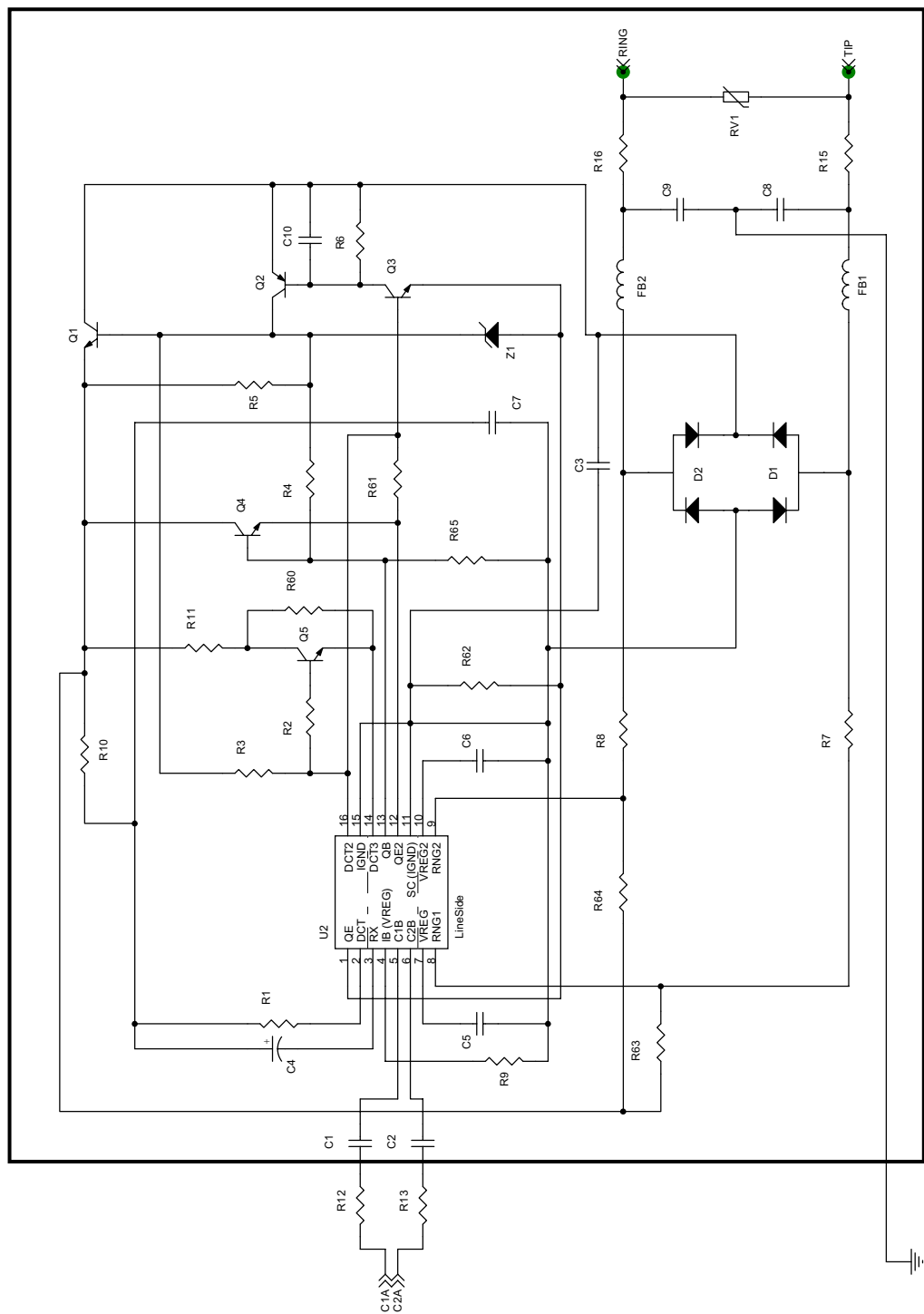
Figure 13. Si3052 and Si3017/11/18 Typical Application Schematic (1 of 2)
