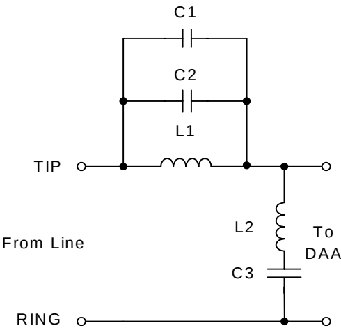
Figure 27. Billing Tone Filter
