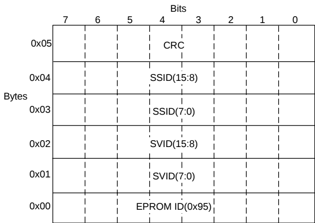
Figure 20. EPROM Map
