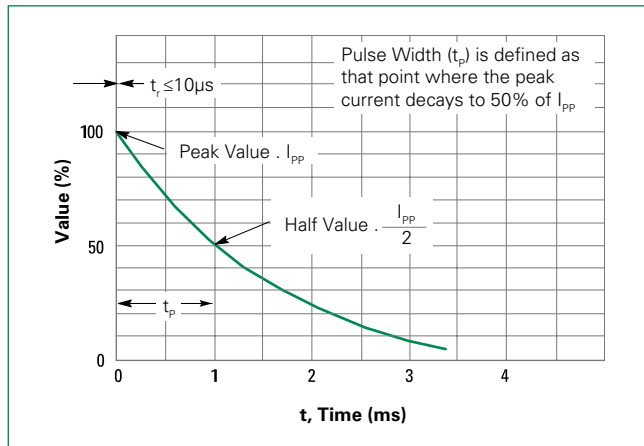
Figure 2. Pulse Waveform
