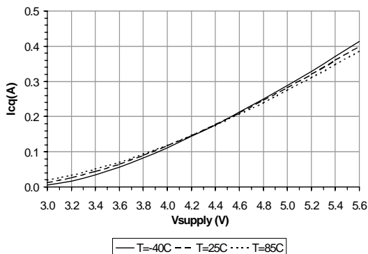
Icq (DC Bias Point) vs Vsupply (V+ and Vpc)
