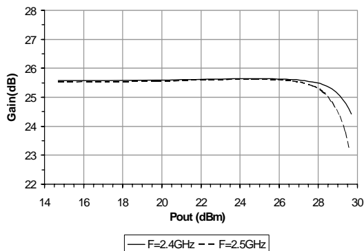
Gain vs Pout, T=25C
