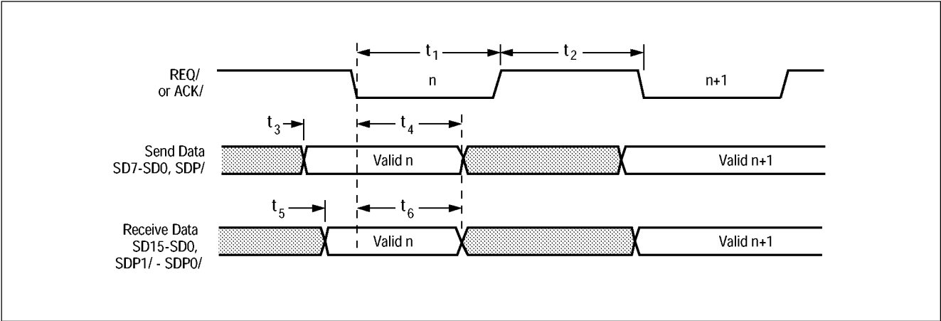
Figure 6-42: Initiator and Target Synchronous Transfers
