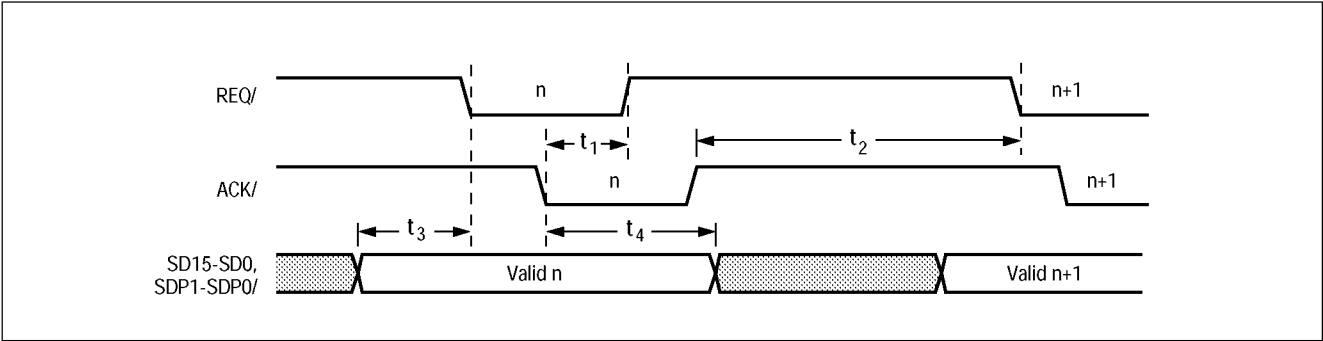
Figure 6-40: Target Asynchronous Send Waveforms
