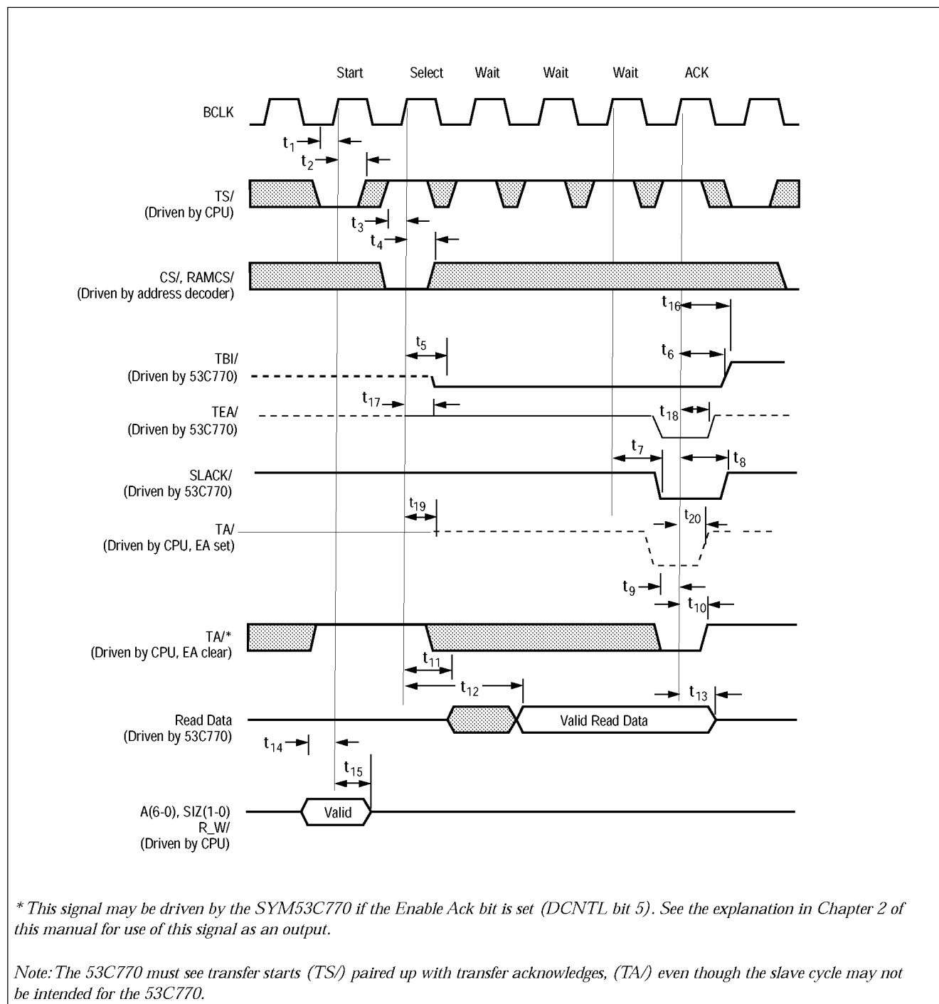
Figure 6-17: Bus Mode 2 Slave Read Waveforms
