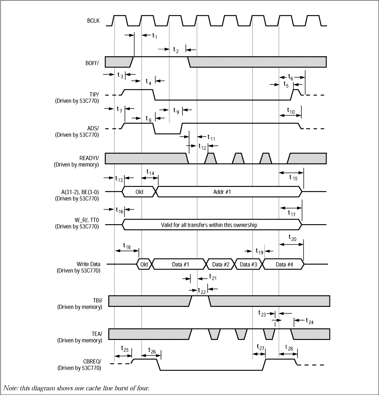
Figure 6-37: Bus Mode 4 Bus Master Write (Cache Line Burst)
