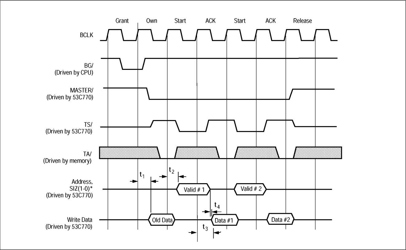
Figure 6-26: Mux Mode Write Cycle (Non-Cache Line Burst)
