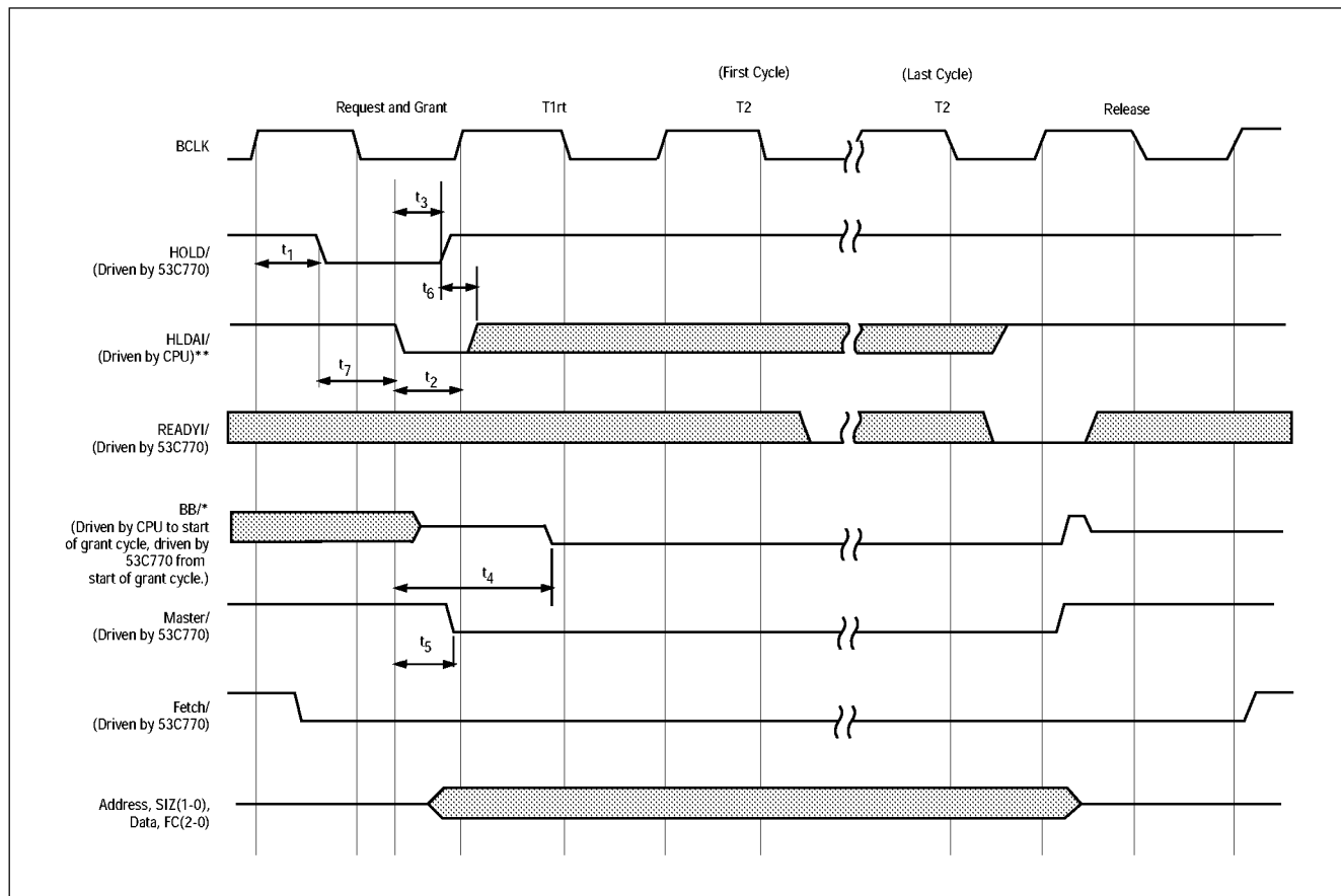
Figure 6-31: Bus Mode 3 and 4 Fast Arbitration
