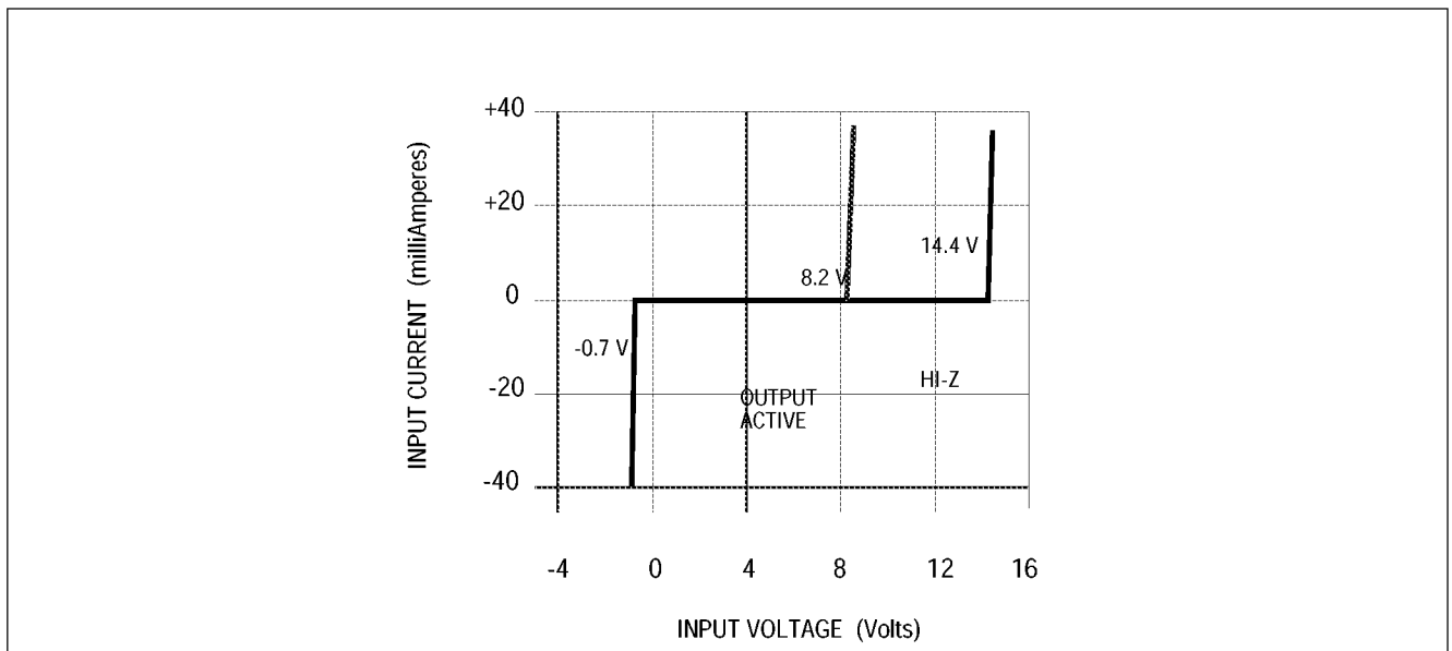
Figure 6-4: Input current as a Function of Input Voltage
