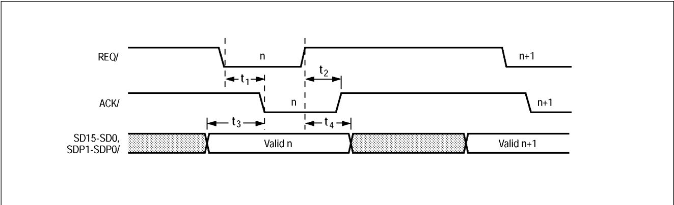
Figure 6-38: Initiator Asynchronous Send
