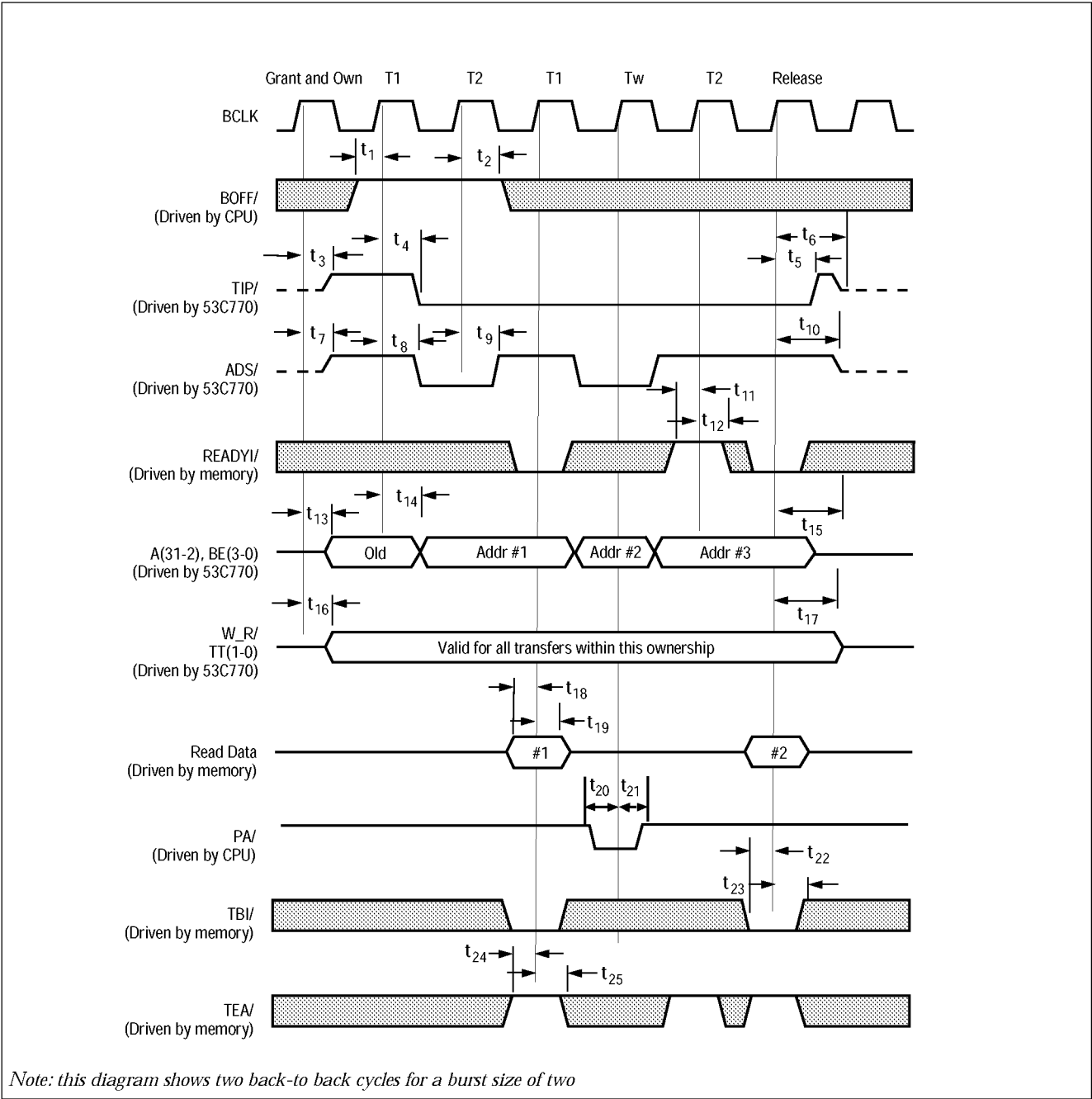
Figure 6-33: Bus Mode 3 and 4 Bus Master Read (Preview of Address)
