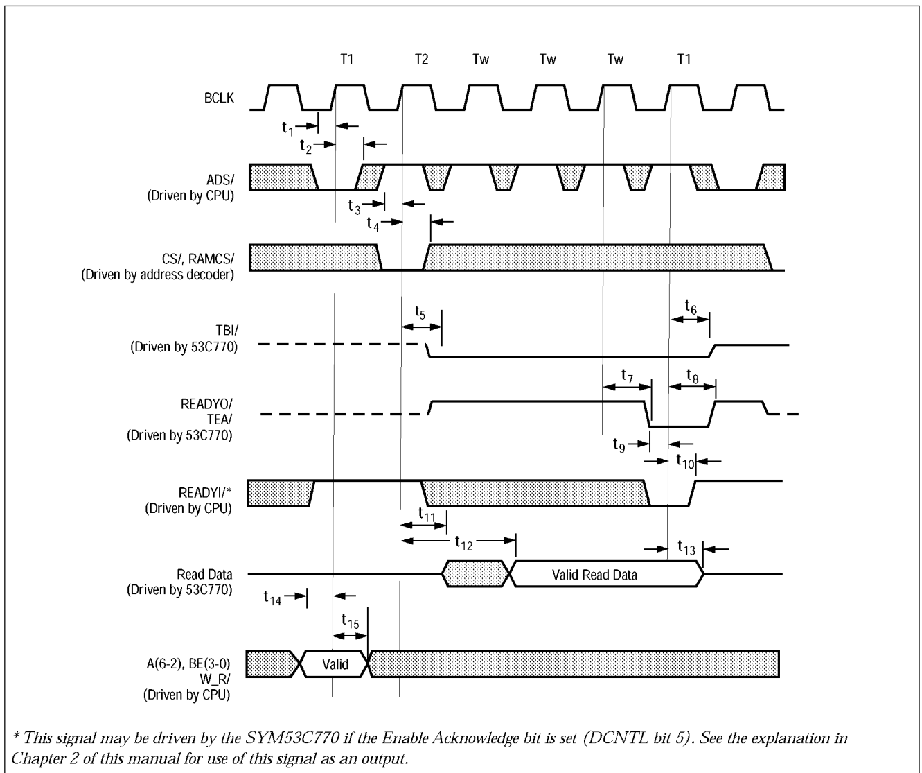
Figure 6-28: Bus Mode 3 and 4 Slave Read Cycle
