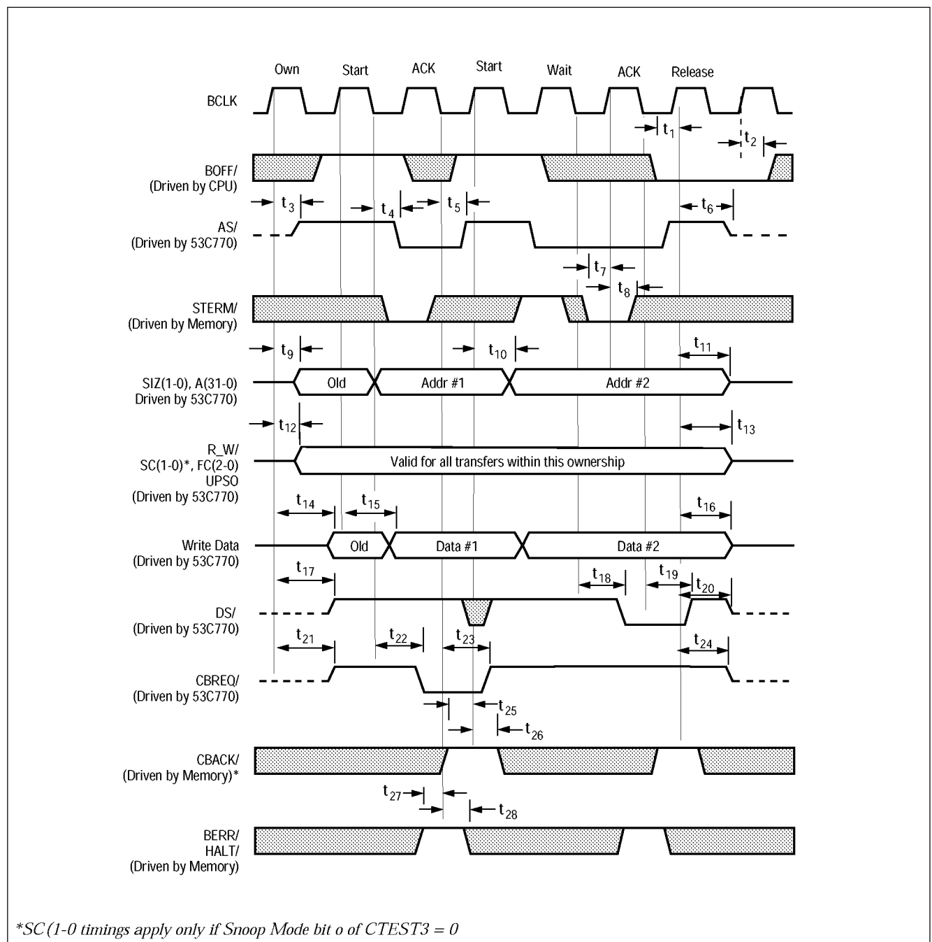
Figure 6-15: Bus Mode 1 Bus Master Write (Cache Line Burst Requested but not Acknowledged)
