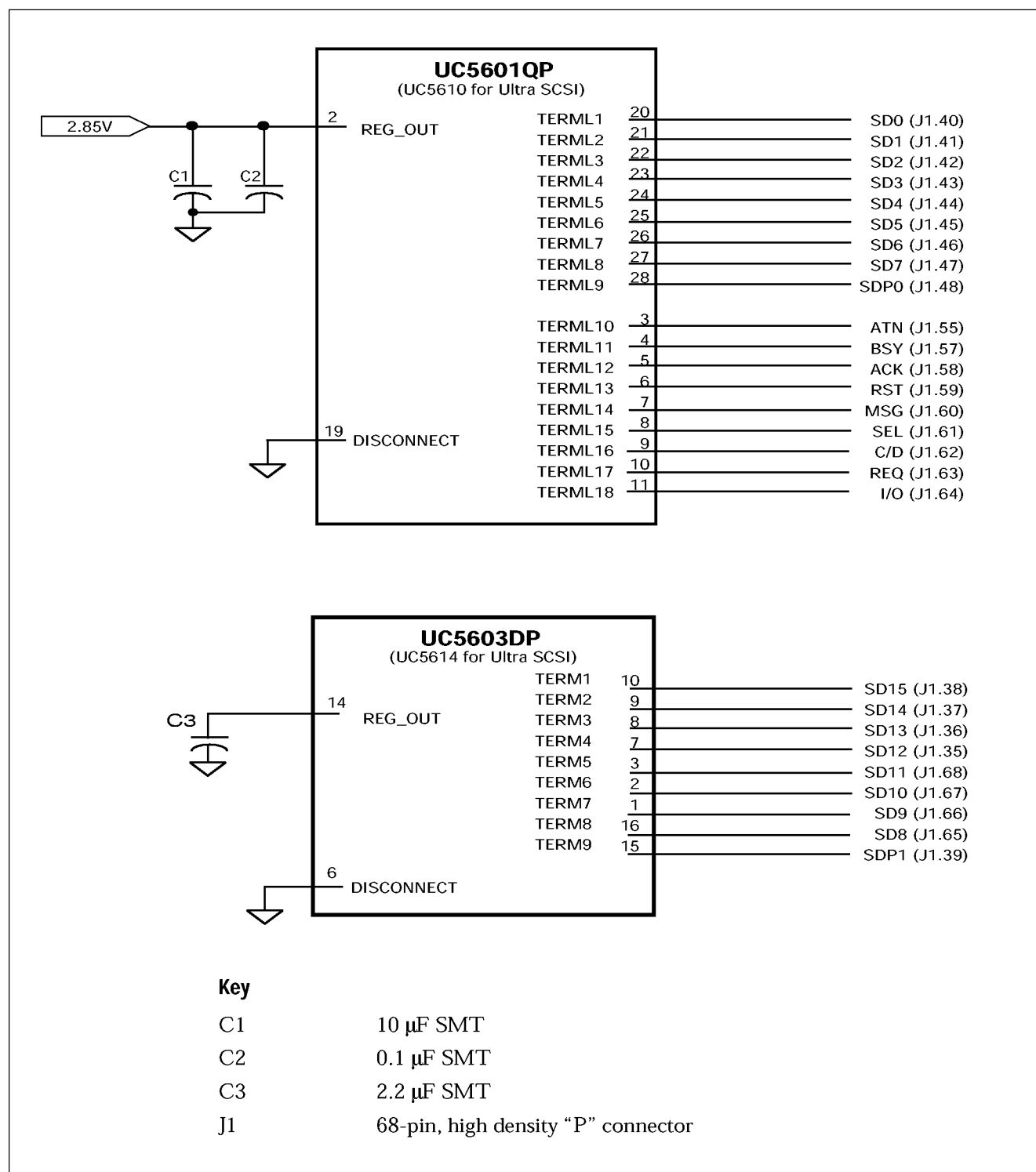
Figure 2-7: Regulated Termination
