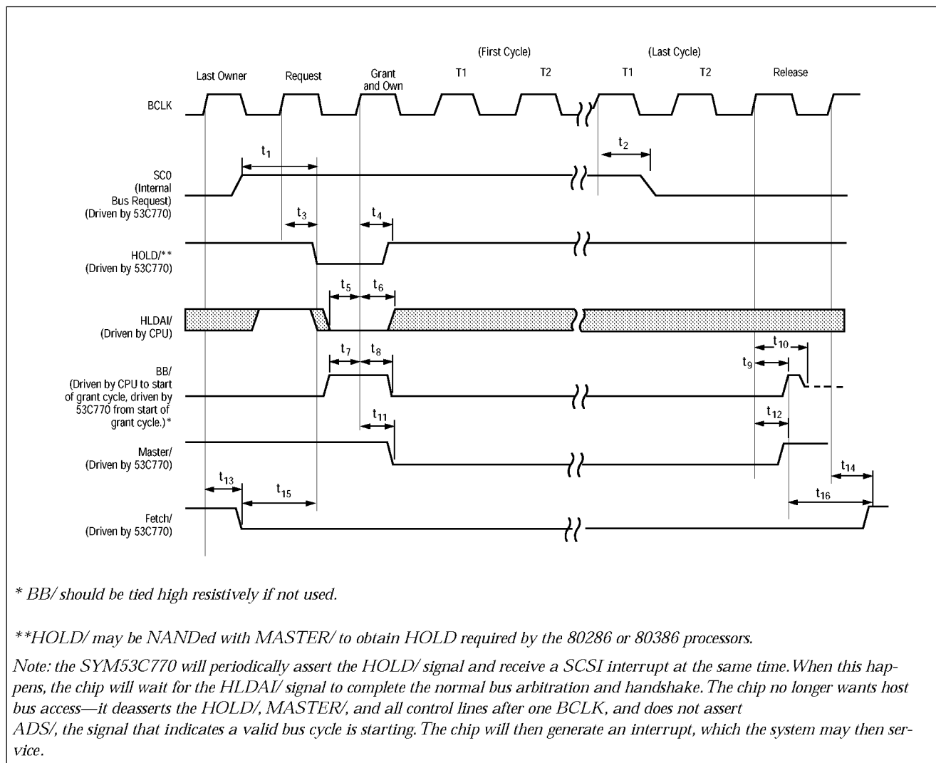
Figure 6-30: Bus Modes 3 and 4 Host Bus Arbitration
