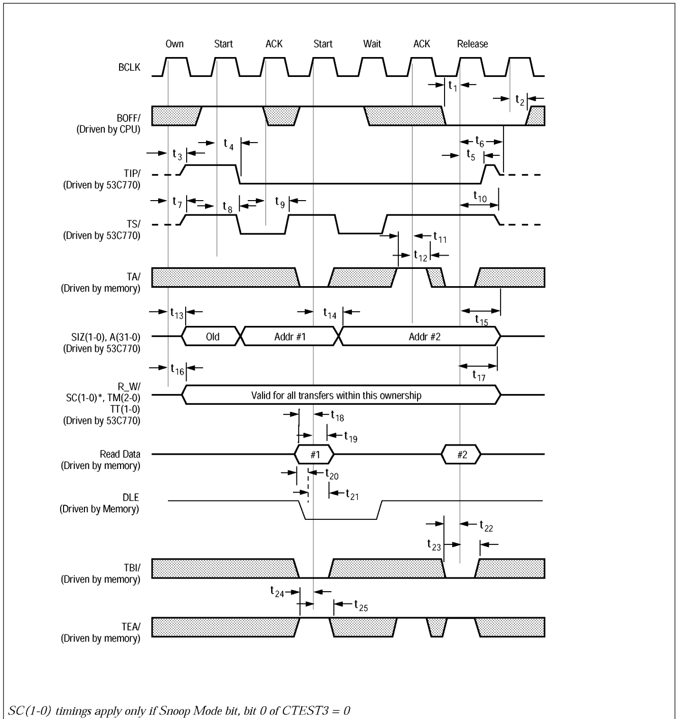
Figure 6-21: Bus Mode 2 Bus Master Read (Cache Line Burst Requested but not Acknowledged)
