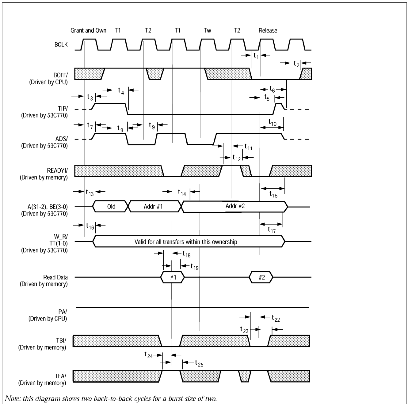
Figure 6-32: Bus Mode 3 and 4 Bus Master Read (Non-Preview of Address)
