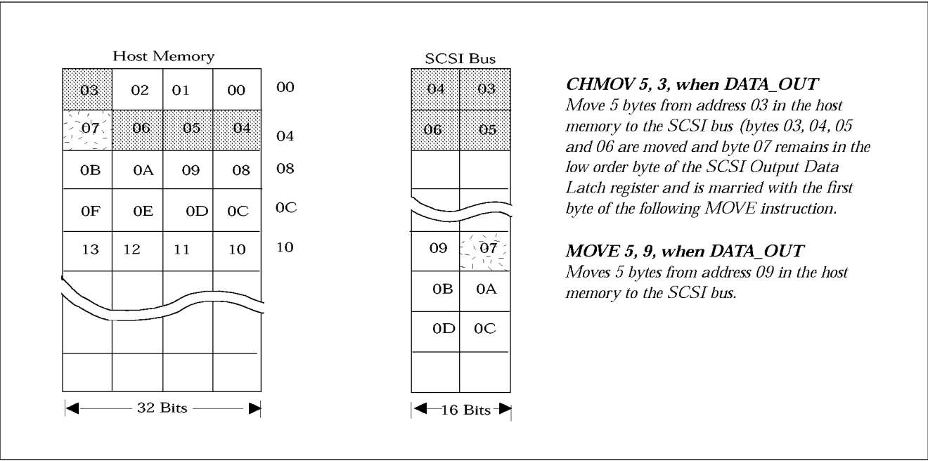
Figure 5-2: Block Move and Chained Block Move Instructions
