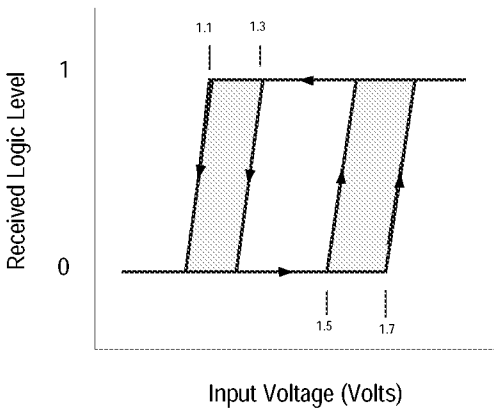
Figure 6-3: Hysteresis of SCSI Receiver
