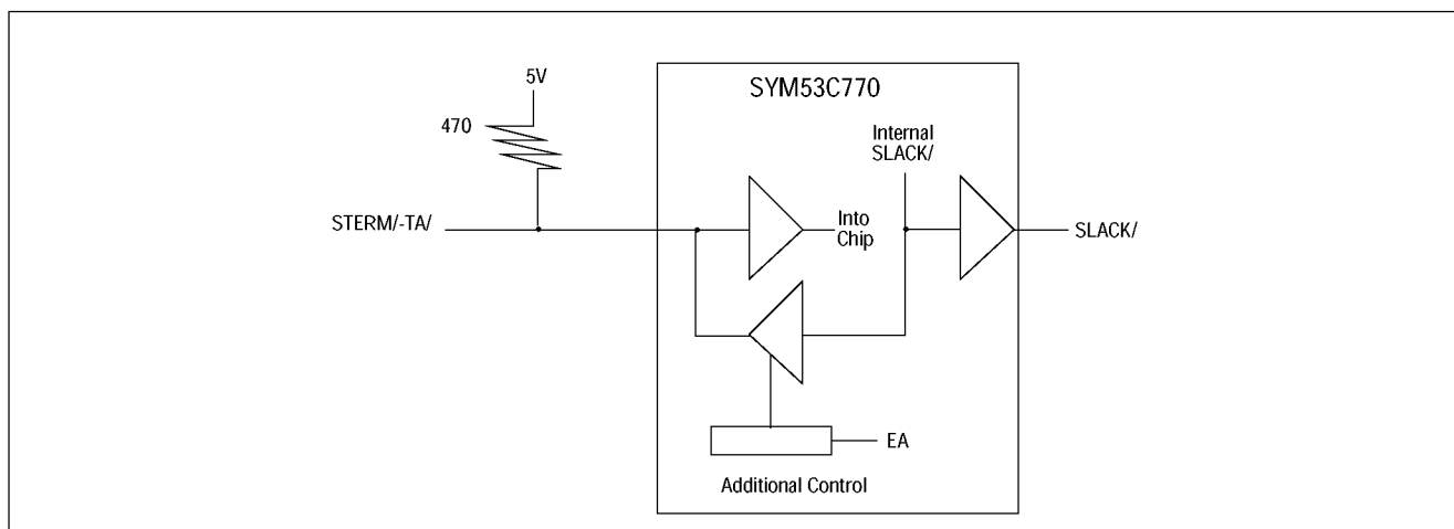
Figure 2-5: Bidirectional STERM/, EA bit set
