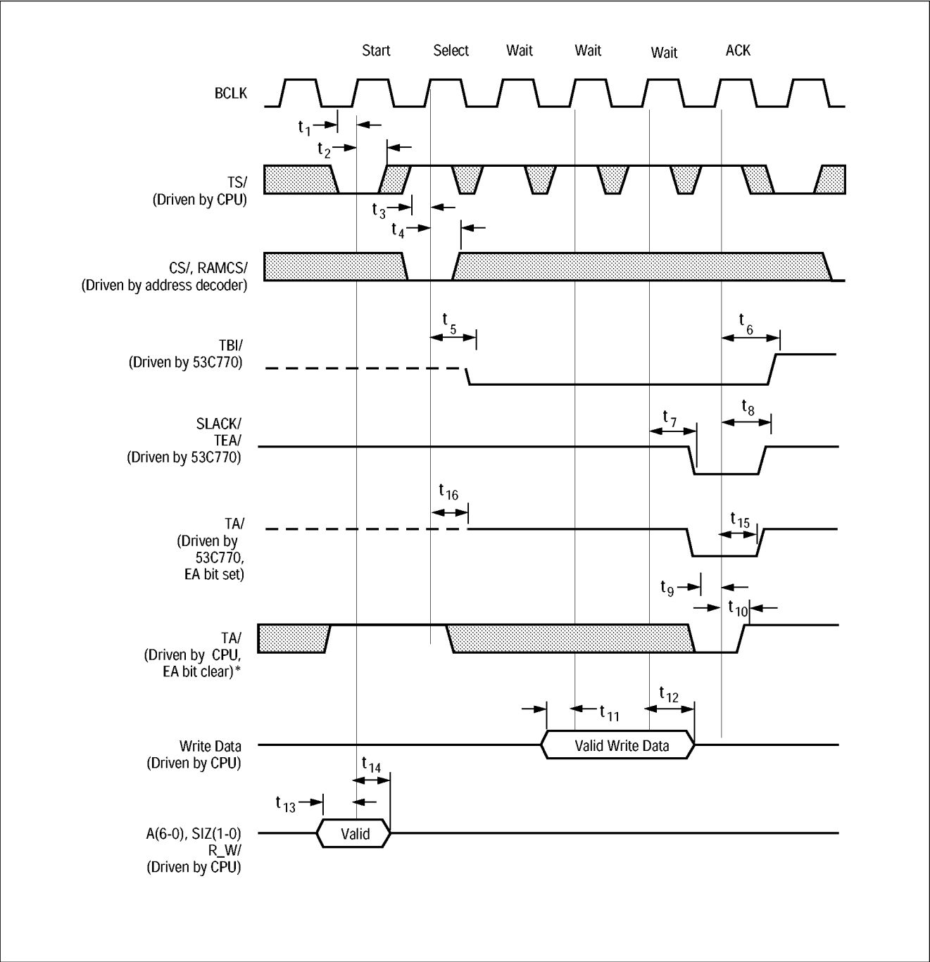
Figure 6-18: Bus Mode 2 Slave Write Waveforms
