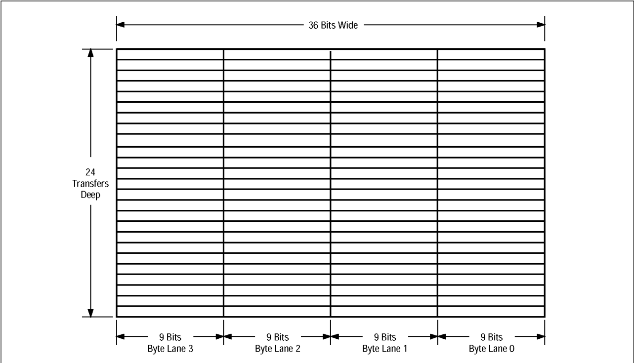
Figure 2-1: DMA FIFO Byte Lanes
