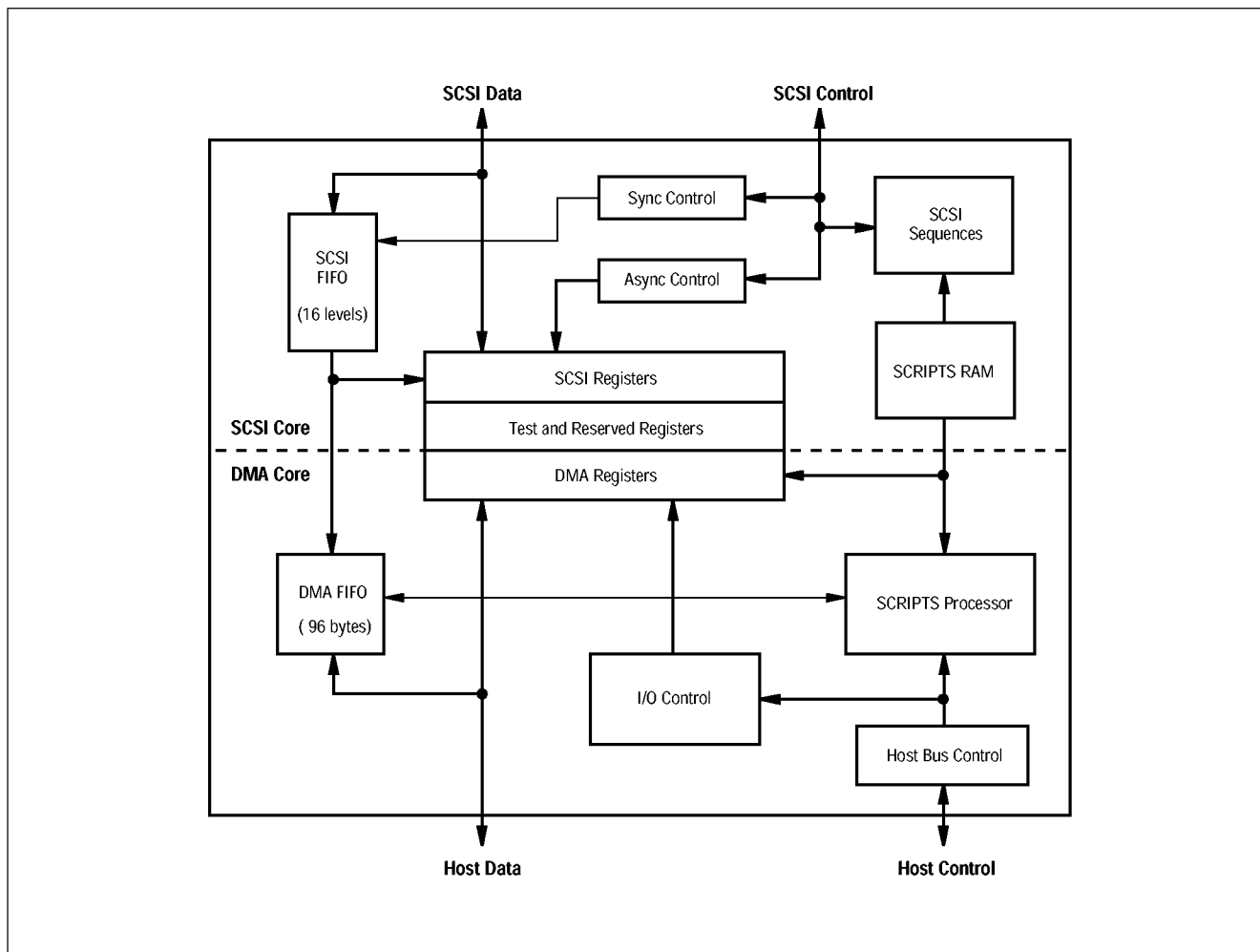
Figure 1-1: SYM53C770 Block Diagram
