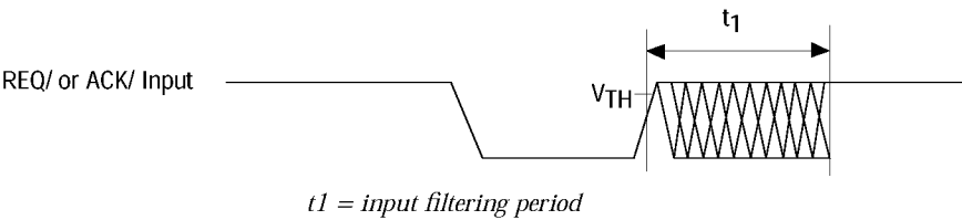
Figure 6-2: SCSI Input Filtering
