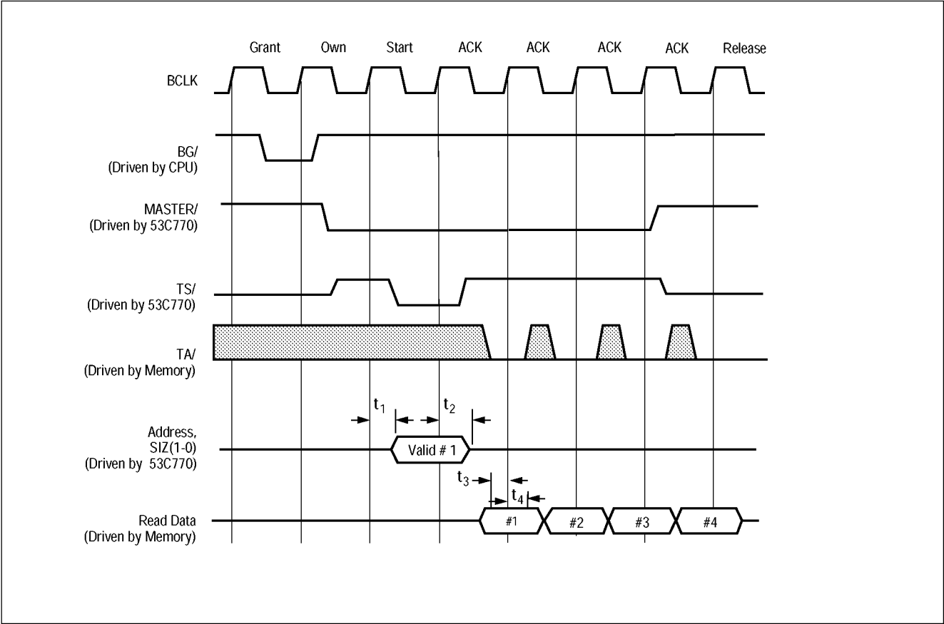
Figure 6-25: Mux Mode Read Cycle (Cache Line Burst)
