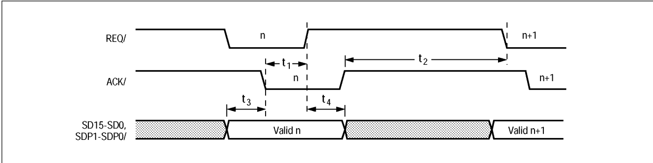
Figure 6-41: Target Asynchronous Receive
