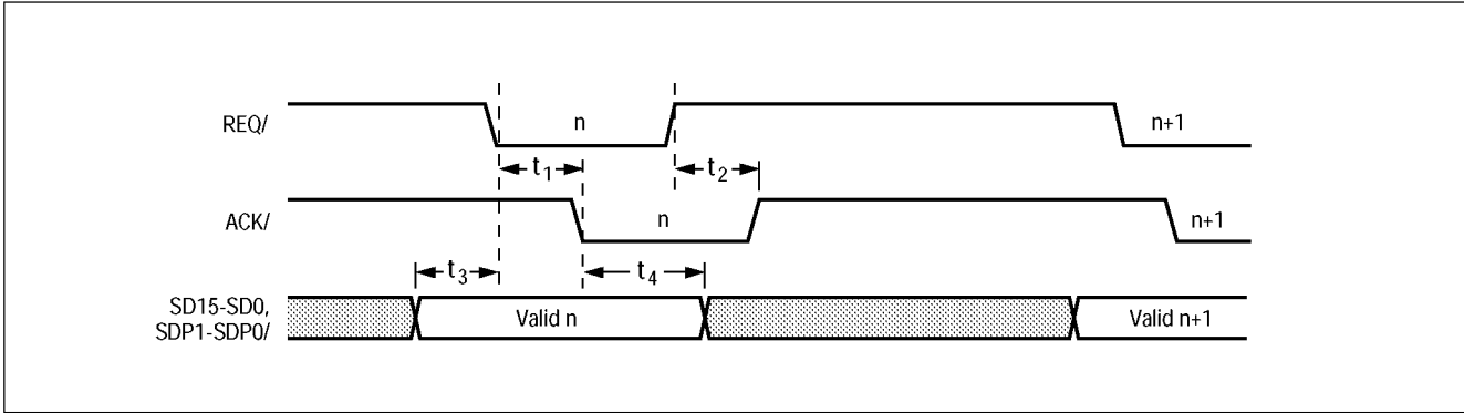
Figure 6-39: Initiator Asynchronous Receive
