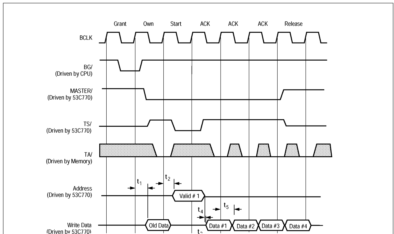
Figure 6-27: Mux Mode Write Cycle (Cache Line Burst)
