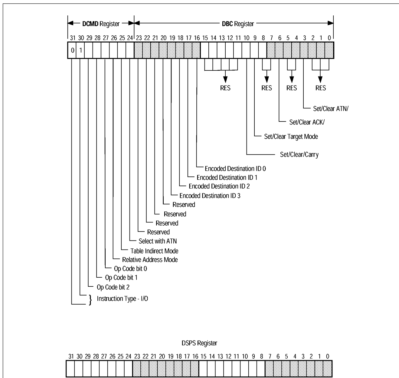
Figure 5-3: I/O Instruction Register
