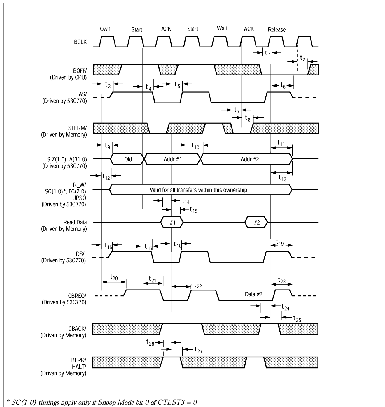
Figure 6-13: Bus Mode 1 Bus Master Read (Cache Line Burst Requested but not Acknowledged)
