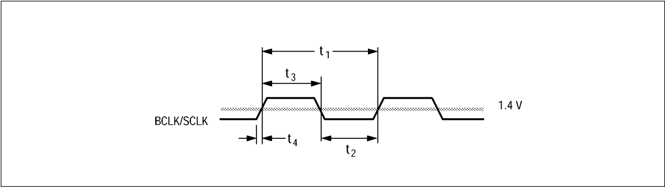
Figure 6-6: Clock Waveform
