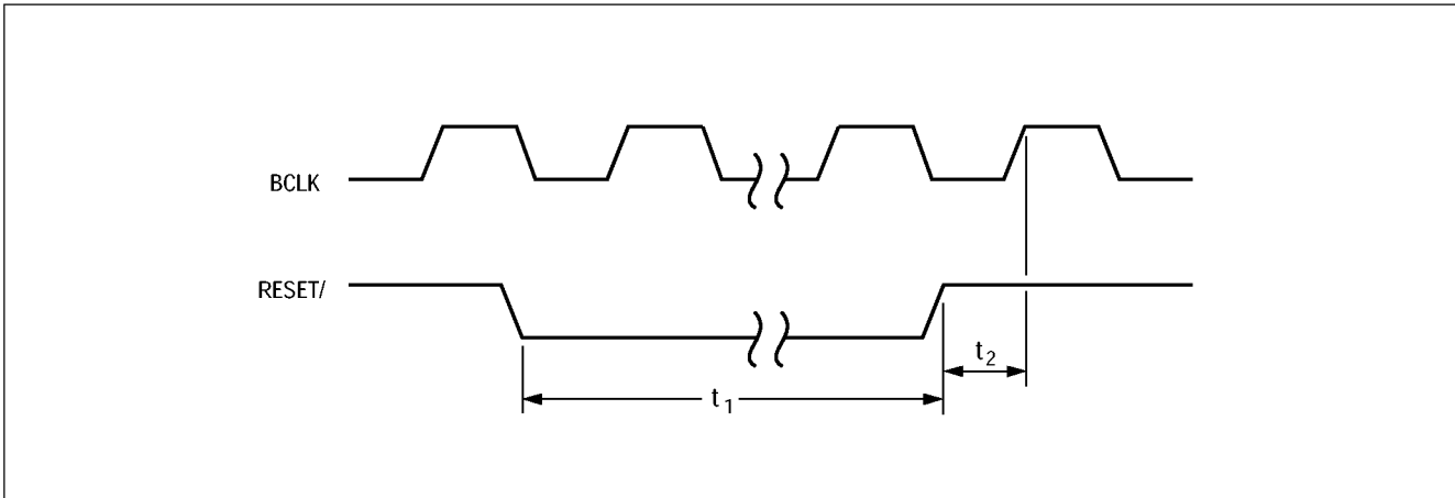
Figure 6-7: Reset Input Waveforms
