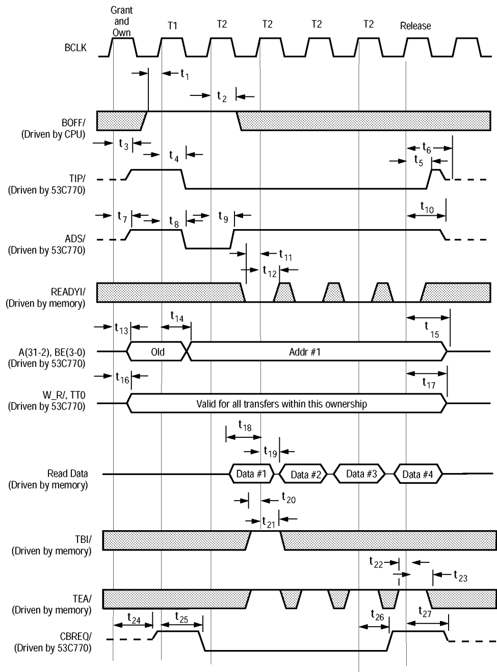
Figure 6-34: Bus Mode 4 Bus Master Read (Cache Line Burst)
