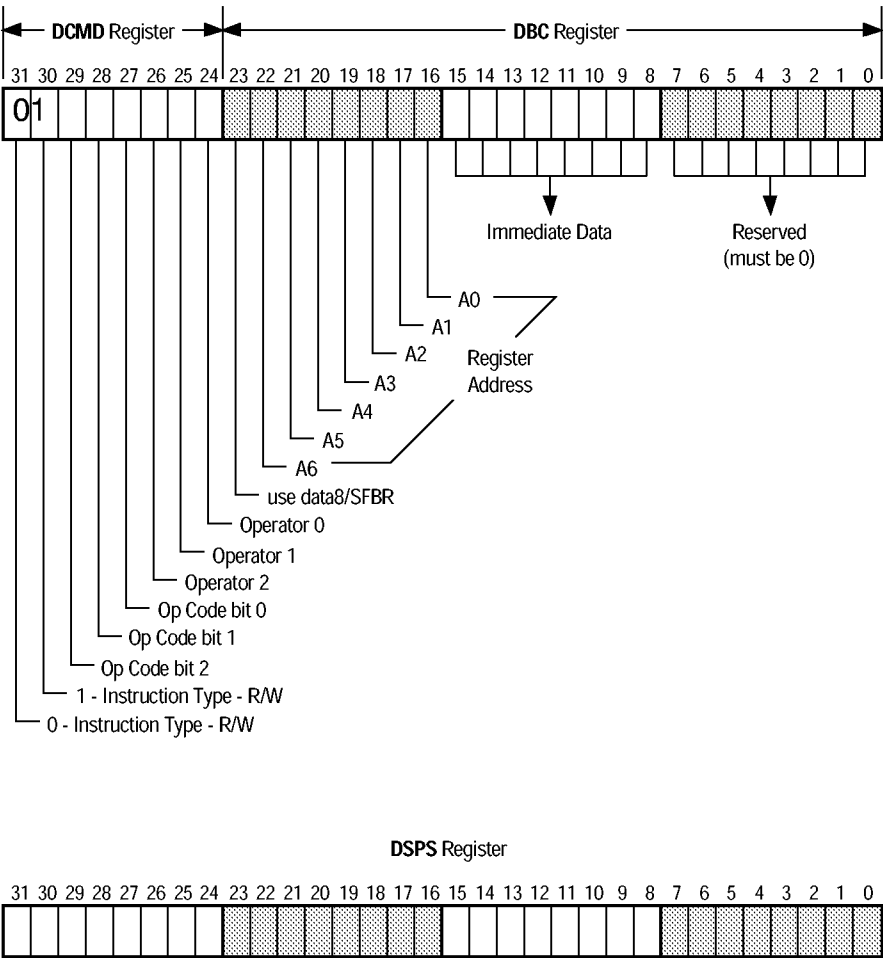
Figure 5-4: Read/Write Instruction Register
