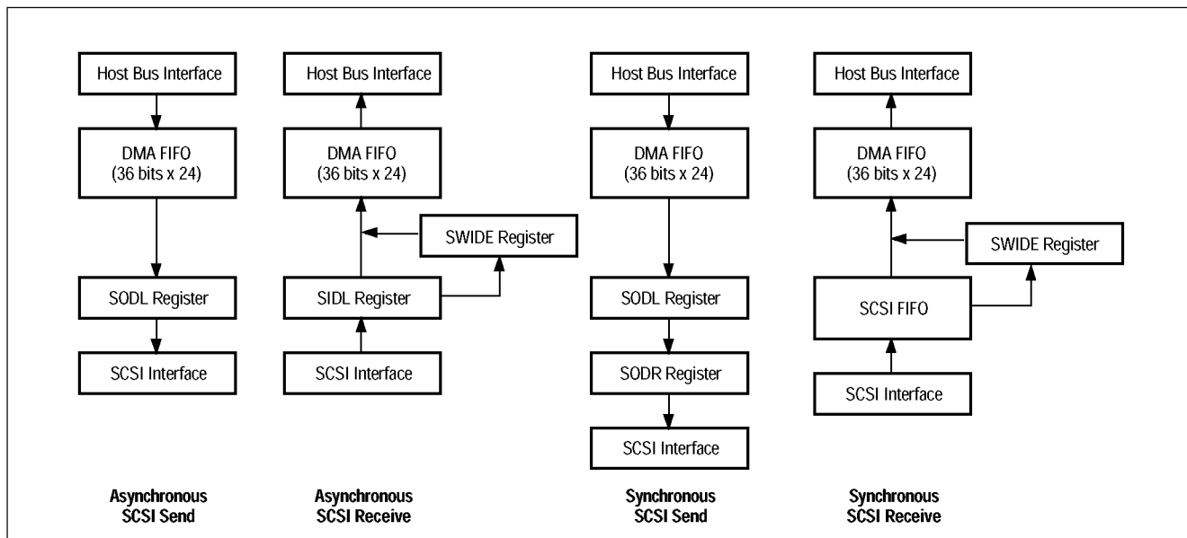
Figure 2-2: SYM53C770 Data Paths
