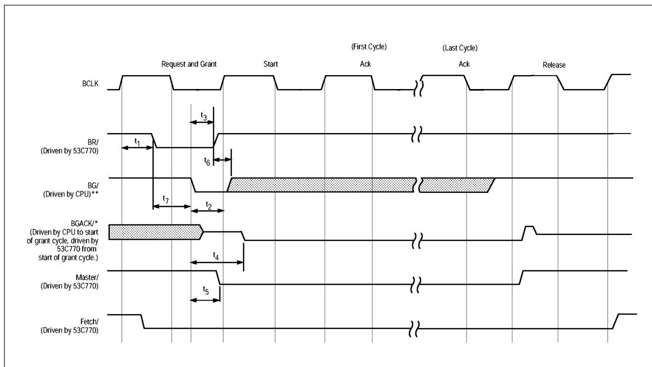
Figure 6-12: Bus Mode 1 Fast Arbitration
