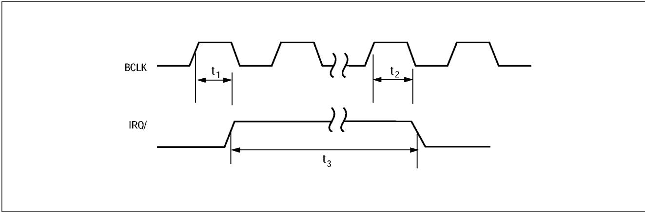
Figure 6-8: Interrupt Output Waveforms
