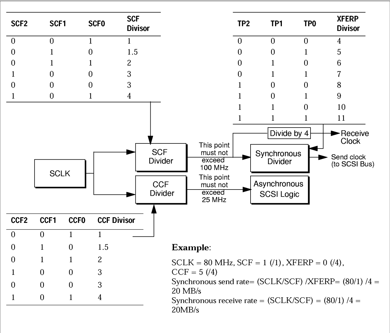
Figure 2-8: Determining the Synchronous Transfer Rate
