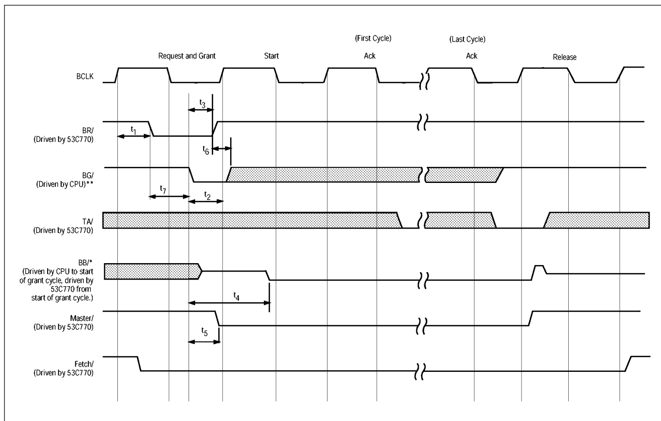
Figure 6-20: Bus Mode 2 Fast Arbitration
