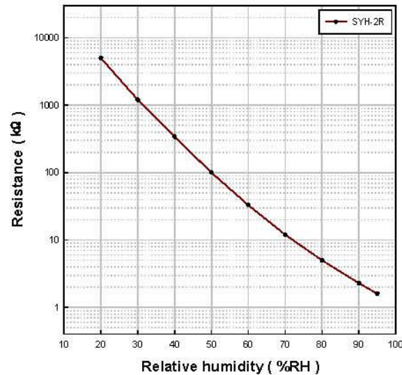
Fig. 2. Standard characteristics
