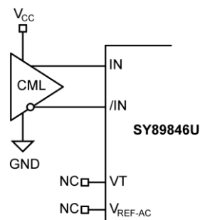
Figure 4c. CML Interface (DC-Coupled)
