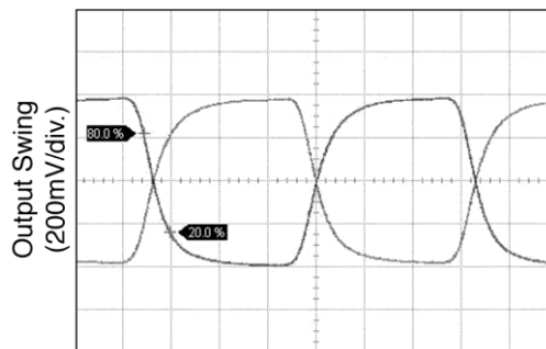
TIME (300ps/div.)
