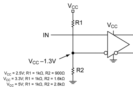
Figure 1. Single-Ended Input (Terminating unused Input)
