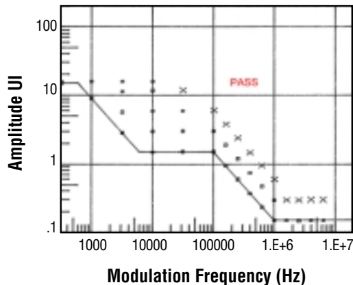
OC-48 Jitter Tolerance
