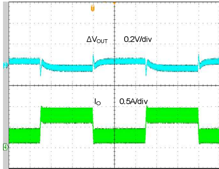
Load Transient ( V_{IN}=24V , V_{OUT}=12V , I_O=0.25 \sim 0.75A )
