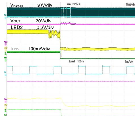
Open LED Protection (Open LED2)
